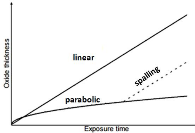
Figure 2-3. Oxidation kinetics for linear and parabolic oxidation [34]
