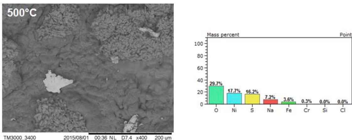
Figure 7-16(b). SEM- EDS values for SW1600 at \text{SO}_2/\text{HCl} = 0.3 , 500°C
