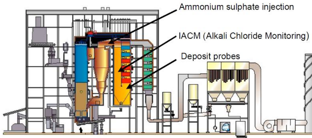
Figure 3-3. Vattenfall Chlorout concept [80].
