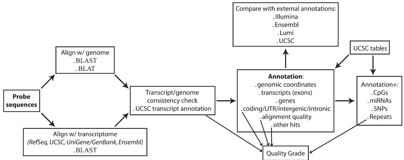
Figure 1. Annotation pipeline. Schematics of the computational pipeline flow—see Methods section for details.
