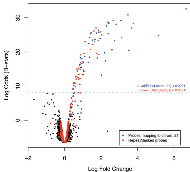
Figure 4. Effect of repetitive sequences on gene expression measurements. Volcano plot ( y -axis: empirical Bayes log-odds of differential expression; x -axis: \log_2 fold change in expression) comparing the expression of human transcripts in livers between Tc1 mice carrying a human chromosome 21 and their wild-type litter-mates (Tc0). Blue dots depict probes targeting genes on human chromosome 21 and red dots probes comprising human RepeatMasker sequences. The dashed line is an arbitrary cut-off for differential expression based on the assumption that there are no human sequences transcribed in the wild-type mouse and, therefore, no human transcript should be overexpressed in Tc0. The P -values (Fisher's exact test) show that the numbers of differentially expressed transcripts from human chromosome 21 (blue) and comprising human repeats (red) are both highly significant.
