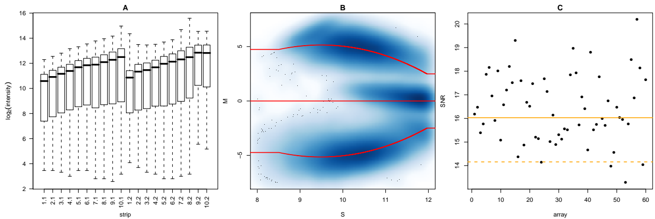
Fig. 1. A) Plot of the \log_2 alleleB (green) intensity by strip (labelled by Row.Column position) which steadily increases from rows 1 to 10 down the BeadChip. This effect is less prominent in the allele A (red) channel (data not shown). The source of this trend is related to the way post-hybridization reagents are applied to the BeadChip and scan order, and its presence motivates strip-level normalization. B) A smoothed scatter plot of M versus S for a typical array, where darker regions indicate a higher density of points. This plot shows intensity dependent effects in M which vary for the AA and BB genotypes, and motivate the three-component mixture model in CRLMM. The curves represent the smoothing splines that model this effect. C) SNR for 60 arrays, with the median (solid line) and median - median absolute deviation (dashed line) SNR values plotted. Lower scores correspond to poorer separation between the genotype clouds depicted in panel B. This metric can be used to flag low-quality arrays to exclude from further analysis.
