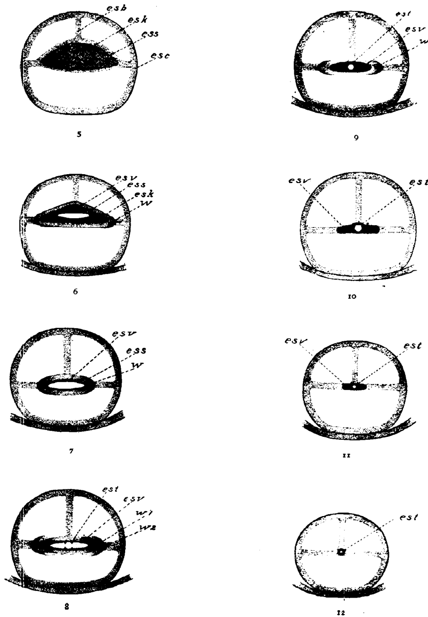
Fig. 5-12 Diagrammatic sections of siphuncle of Cameroceras brainerdi Whitfield (sp.). esb , endosiphoblade; esc , endosiphocylinder; esk , endosiphococone; ess , endosiphosheath; est , endosiphotube; esv , endosiphocoleon; w , wing; w 1 , younger wing; w 2 , older wing. In figure 11, the endosiphocoleon is shaded too dark.
