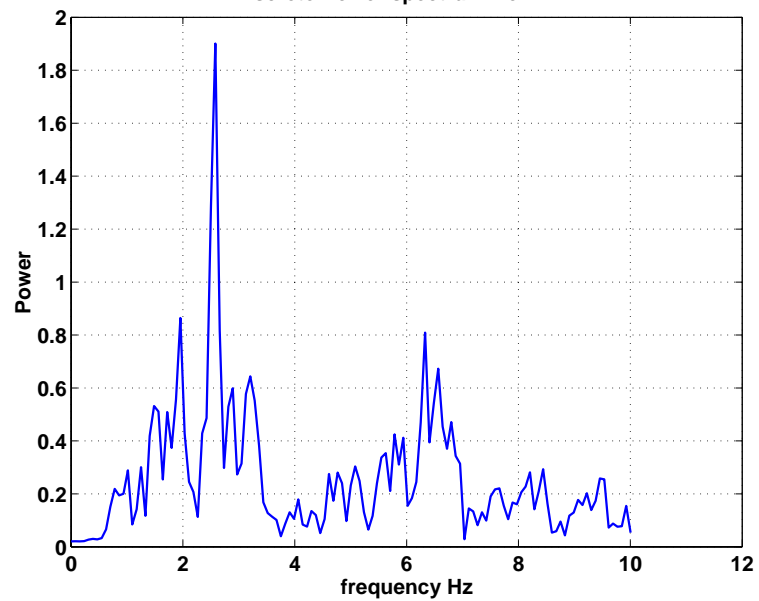
Discrete Power spectrum from FFT
