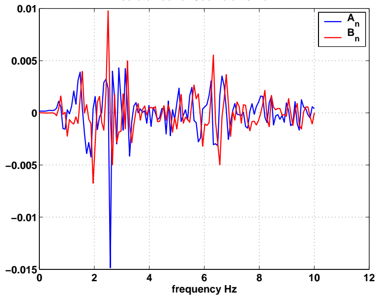
Discrete Fourier Coefficients from FFT
