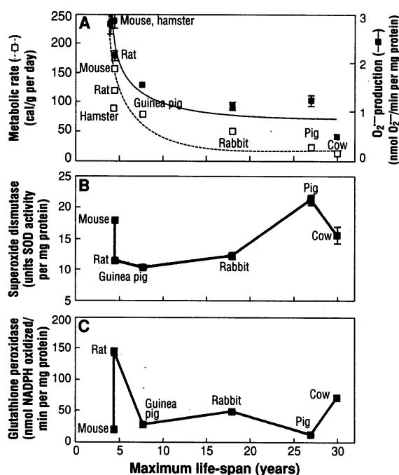
Fig. 2. Comparison of maximum life-span (MLS) with (A) metabolic rate and rate of O_2^- generation in submitochondrial particles, (B) total superoxide dismutase activity, and (C) glutathione peroxidase activity, in the heart of different mammalian species. [Adapted from (4) and (29)] MLS shows an inverse relation to metabolic rate (reported as calories consumed per gram of body weight per day) and O_2^- generation, but no relation to antioxidative enzyme activity.
