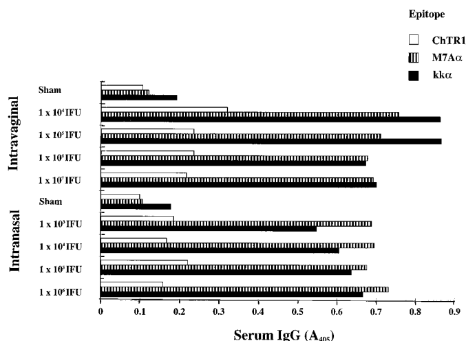
Fig. 4. Serum IgG antibody production in C. trachomatis -infected mice. Eight-week-old female BALB/c mice were inoculated either intranasally or intravaginally with the indicated doses of C. trachomatis MoPn IFUs (31). Thirty-six days (intranasal infection) or 42 days (intravaginal infection) after the inoculation, serum was collected and specific IgG antibody production was determined by ELISA (Fig. 2B). Representative data from individual mice are shown.
