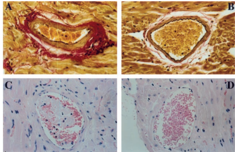
Fig. 3. Blood vessels in mice immunized with C. trachomatis 60-kD CRP-derived peptide (10, 30). (A) Thickening of the arterial wall and perivascular fibrotic changes in mice immunized with ChTR1. The perivascular mononuclear inflammatory cells are apparent. (B) Normal morphology of the cardiac artery in mice immunized with FCA alone. (C) Occlusion of cardiac blood vessels in mice immunized with ChTR1. (D) No occlusions in cardiac blood vessels were seen in control mice immunized with FCA alone. (A and B) Elastic staining for collagen (red) to detect fibrotic changes. (C and D) H&E staining. Magnification, \times 320 .
