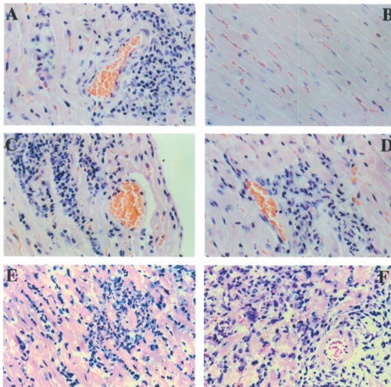
Fig. 1. Inflammatory heart disease in BALB/c mice that were immunized with (A) the endogenous mouse M7A \alpha peptide from the \alpha myosin heavy chain, (B) the control endogenous M7A \beta peptide from the homologous region of the \beta myosin heavy chain, (C) the 60-kD CRP-derived peptide from C. trachomatis (ChTR1), or (D) the 60-kD CRP-derived peptide from C. pneumoniae (ChPN) (10). (E) Adoptive transfer of ChTR1 peptide-induced inflammatory heart disease into nonimmunized recipient mice (27). (F) Induction of inflammatory autoimmune heart disease in BALB/c mice with C. trachomatis DNA-derived CpG containing ODN as adjuvant (25). Perivascular inflammation is apparent in (A), (C), (D), and (F). (B) shows normal heart muscle morphology. Hearts were analyzed 21 days after the initial immunization. Staining was with hematoxylin and eosin (H&E). Magnification: \times 320
