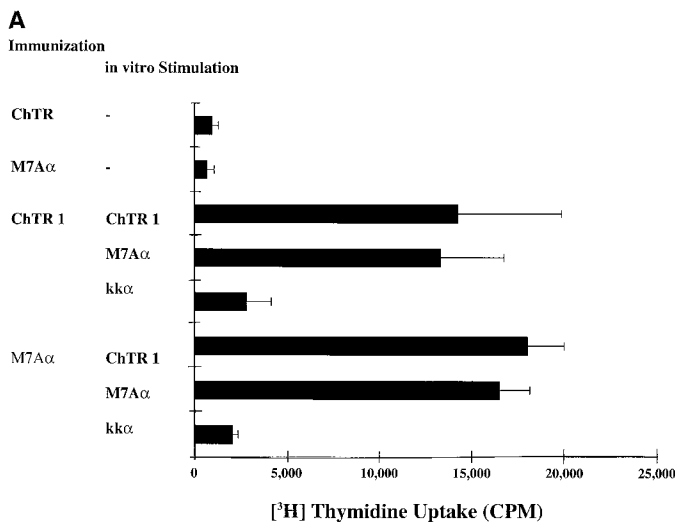
Fig. 2. (A) Splenic T cell proliferation and (B) serum IgG antibody production. (A) Proliferative responses to M7A \alpha , ChTR1, or kk\alpha peptides. Splenic T cells from mice immunized with the indicated peptides were cultured with \gamma -irradiated syngeneic splenocytes pulsed with the indicated peptides (20). [ ^3 H]thymidine uptake (counts per minute) in
