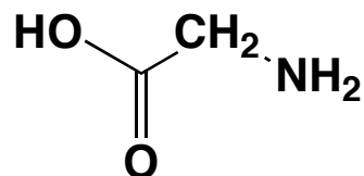
glycine
