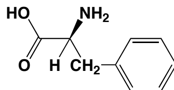
phenylalanine
