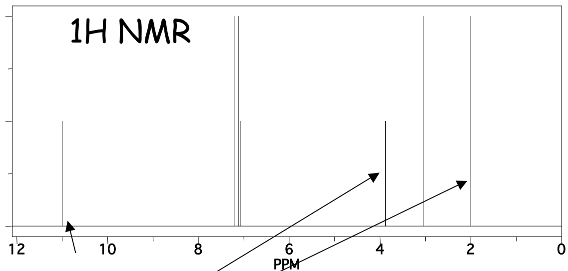
phenylalanine
