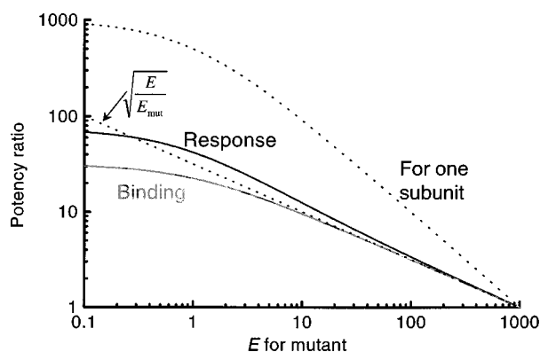
Figure 5 Dependence of potency ratio on E_{mutant} . The shift (relative EC_{50} ) of response and binding curves (solid lines) produced by impairment of gating only, for a receptor that needs two agonist molecules (Scheme 3). The relative EC_{50} is plotted against the efficacy of the mutant, with E=1000 for the wild type.
