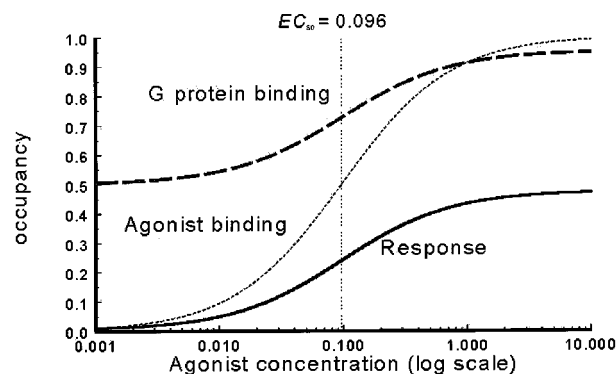
Figure A1 Behaviour of cubic ternary mechanism when G protein concentration is constant (no depletion, excess G). Response (solid curve), binding of agonist (dotted curve, and binding of G protein (dashed curve), as function of [A] ( \mu\text{M} ). This is for the cubic ternary mechanism (Figure 1), with K_A = 1 \mu\text{M} , K_G = 1 \mu\text{M} , E_0 = 0.001 , a = b = g = d = 10 . The EC_{50} , or K_{\text{app}} , from eq.A3, is 0.096 \mu\text{M} .
