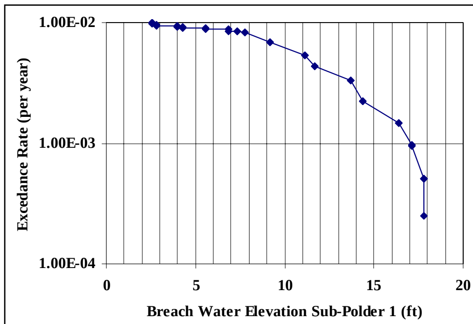
Figure VIII-5. Breach Risk Profile for Sub-Polder 1
