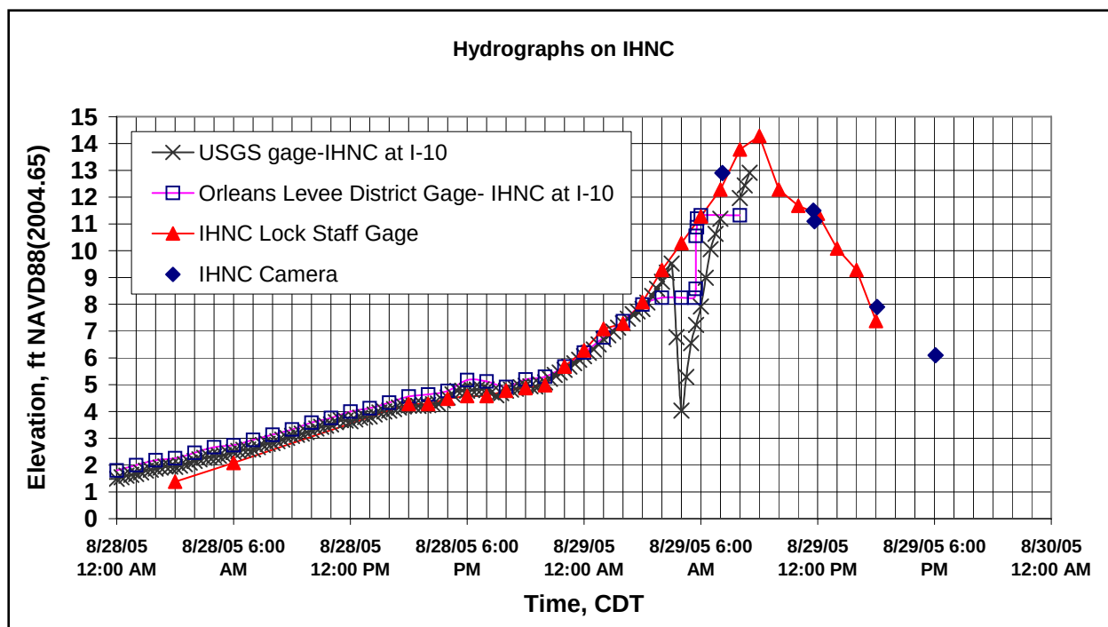
Figure V-6. Stage Hydrographs for IHNC at I-10, and IHNC at Lock
