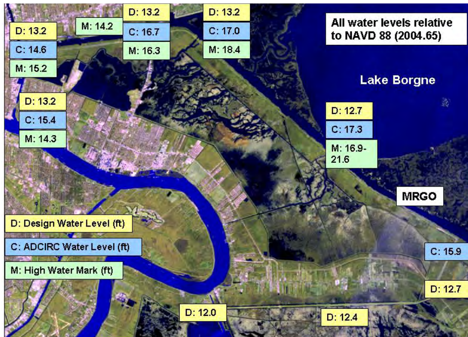
Figure V-47. Water level maxima for eastern St. Bernard Parish hurricane protection system
