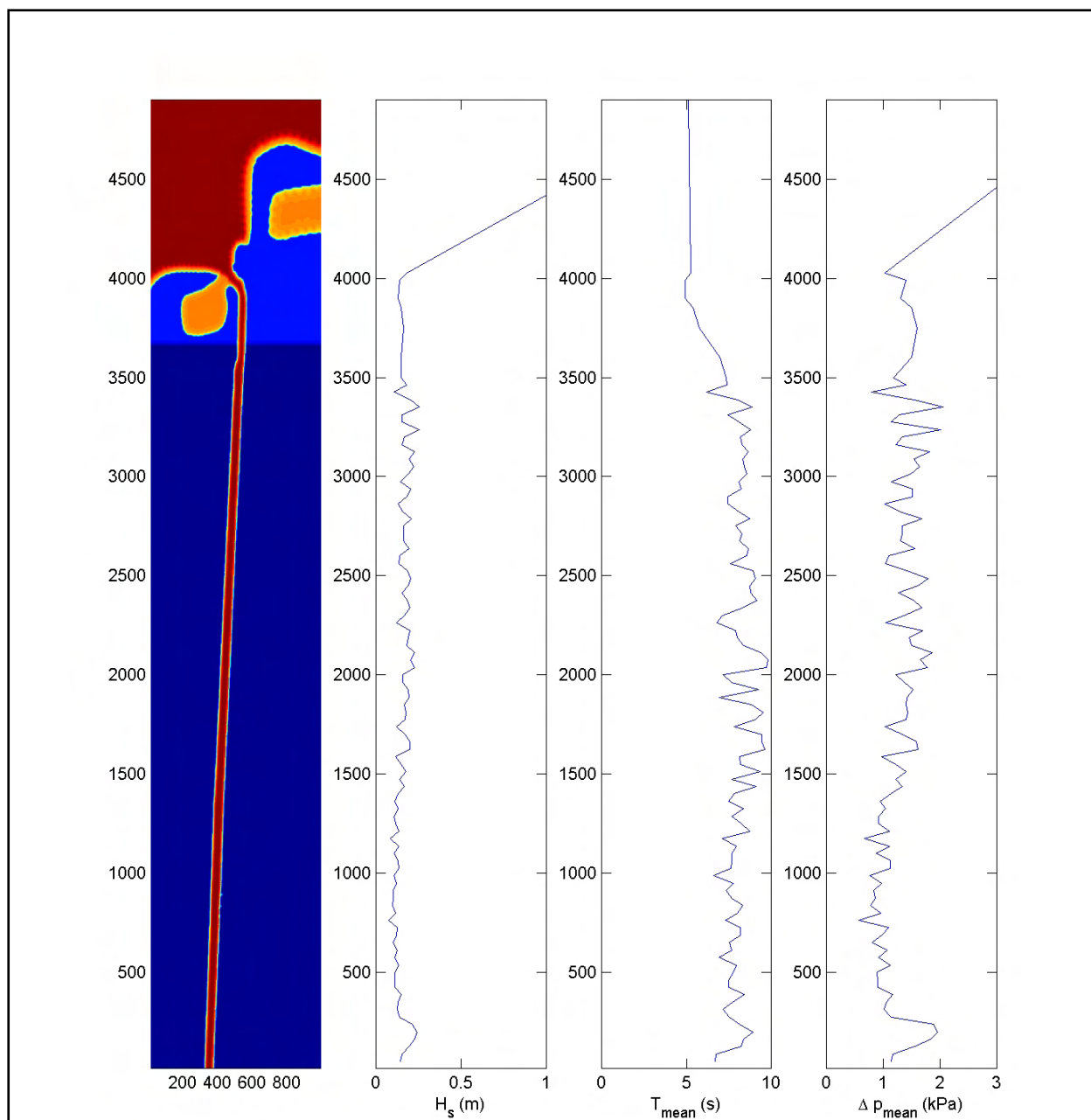
Figure V-60. Canal length profiles for the 0600 simulation
