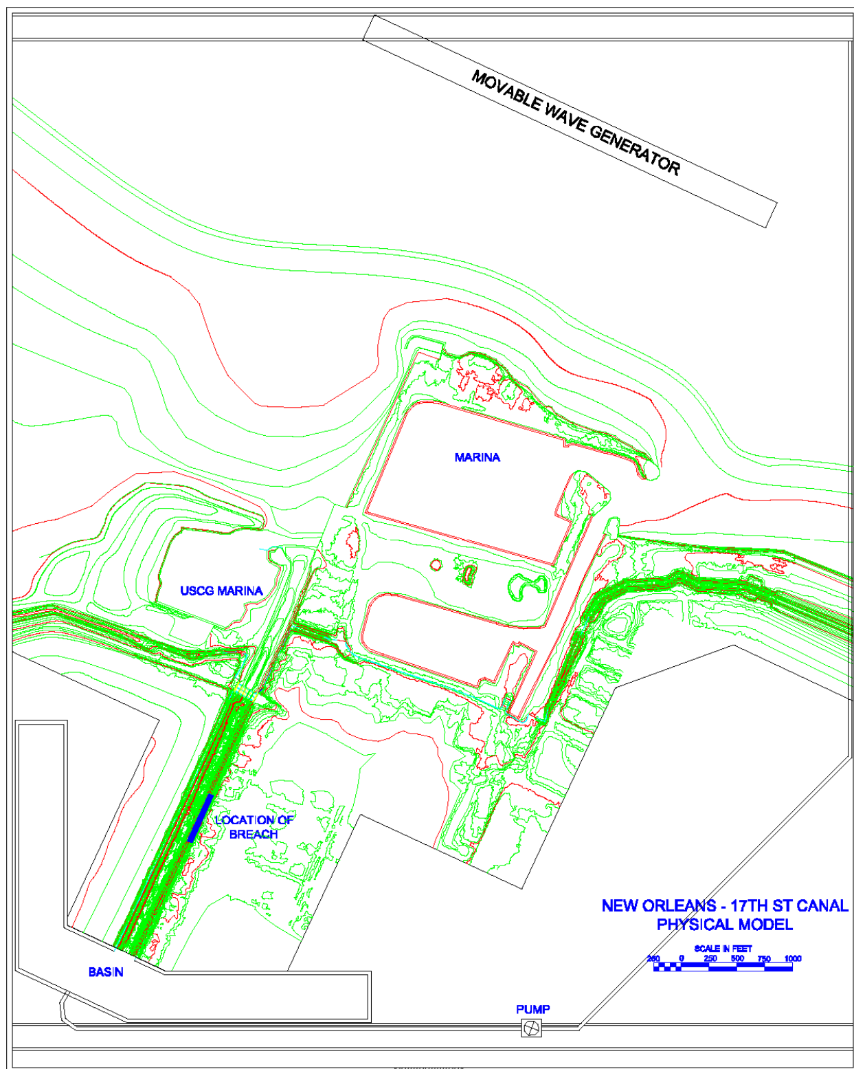
Figure V-79. Layout of 17th St Canal physical model
