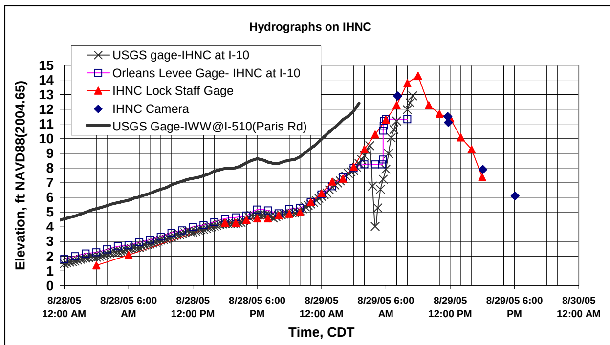
Figure V-27. Hydrographs on the Inner Harbor Navigation Canal (IHNC)
