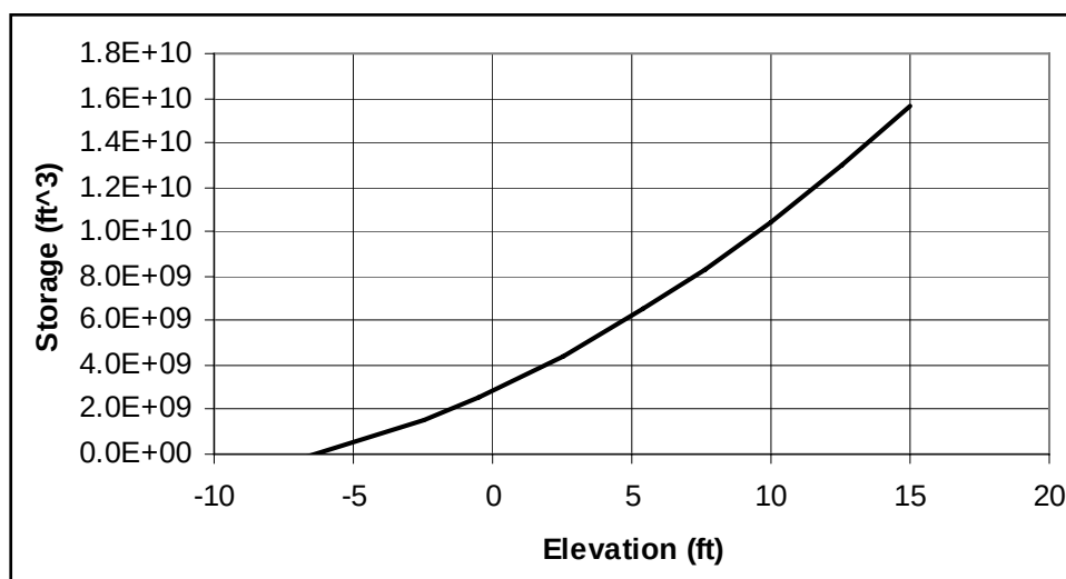
Figure VIII-3. Stage-Storage Curve for Citrus
