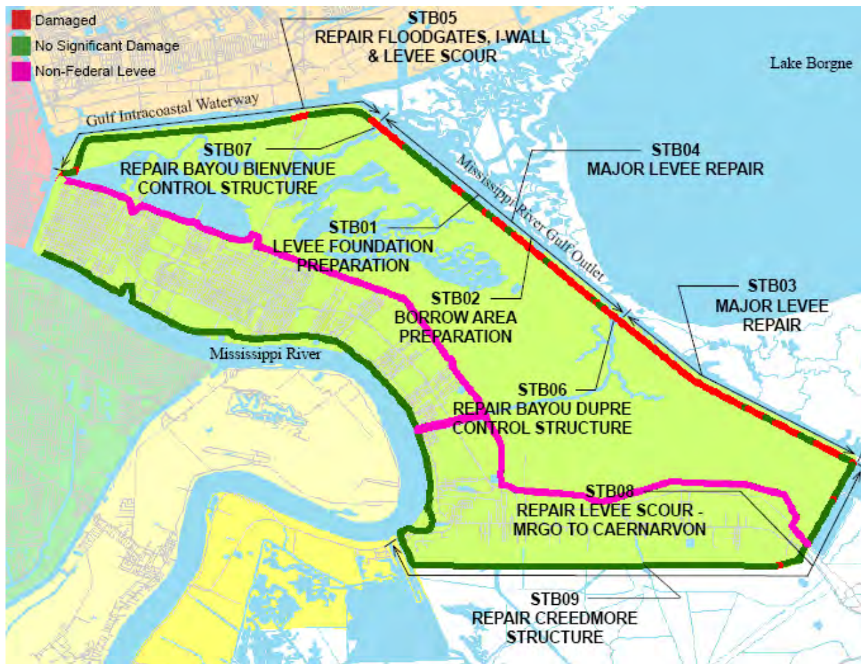
Figure IV-9. Hurricane Protection Project Features – St. Bernard
