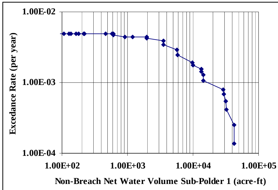
Figure VIII-4. Overtopping Risk Profile for Sub-Polder 1
