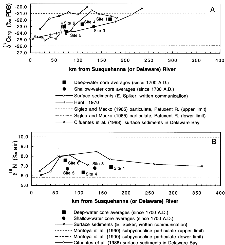
Fig. 4. Values of (A) \delta^{13}C_{org} and (B) \delta^{15}N for transects or ranges of surface sediment samples or particulate matter from Chesapeake Bay, the Patuxent River subestuary (a Chesapeake Bay tributary, see Fig. 1), and Delaware Bay (next major estuary north of Chesapeake Bay on the Atlantic coast of the U.S.). Core site average values since A.D. 1700 are also shown and labeled for comparison. Note that the average site 4 \delta^{15}N value is lower than other deepwater core values (sites 1 and 6) because sediments < \sim 160 yr old were not recovered at that site.
