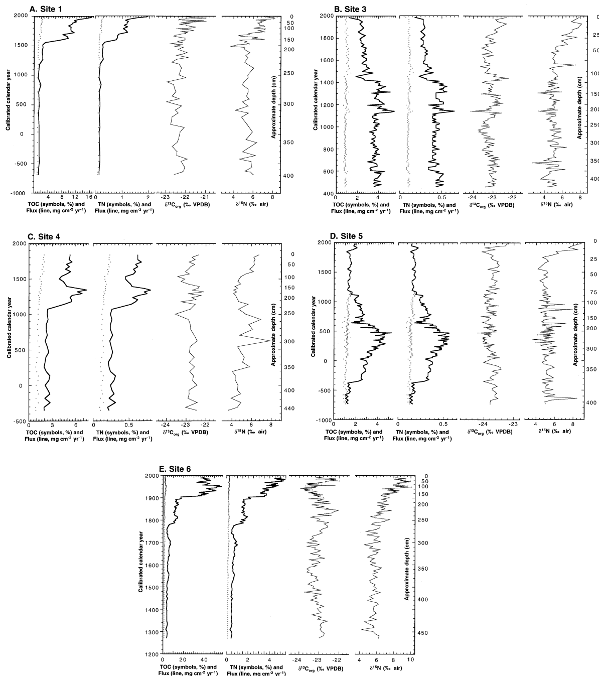
Fig. 2. Plots of sediment TOC and flux, TN and flux, \delta^{13}\text{C}_{\text{org}} and \delta^{15}\text{N} vs. calendar year and depth for cores from (A) site 1, (B) site 3, (C) site 4, (D) site 5, and (E) site 6. Calendar years are A.D. (negative values = B.C.). Depth scales on right y-axes are non-linear.
