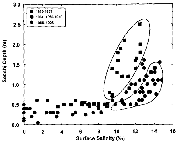
Fig. 4. Summer (July) Secchi depth measurements from data collected between 1936 and 1995 displayed as a function of salinity for the oligohaline and mesohaline regions of the Patuxent River estuary. Encircled data indicate Secchi depths in the early and more recent periods in the mesohaline portion of the estuary. This figure was adapted from Heinle et al. (1980). Data from the 1985–1995 period are from the Maryland Department of Natural Resources (2001).
