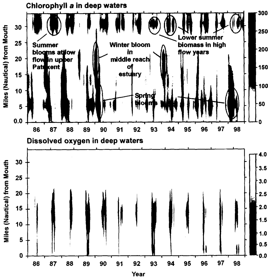
Fig. 10. A time-space plot of water column integrated chlorophyll a ( \text{mg m}^{-2} ) and dissolved oxygen conditions in deep waters ( \text{mg l}^{-1} ) of the Patuxent River estuary from 1986 through 1998. Data are from the Maryland Department of Natural Resources (2001); data were assembled by Hagy (personal communication).
