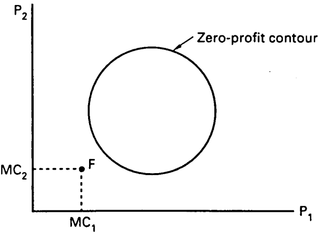
Figure 4.6 Zero-profit contour
