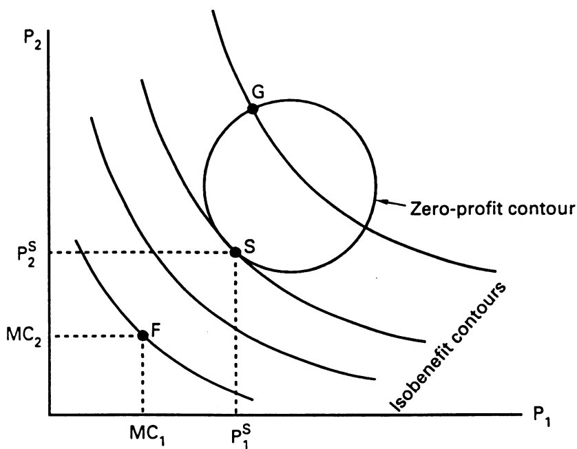
Figure 4.9 Ramsey prices
