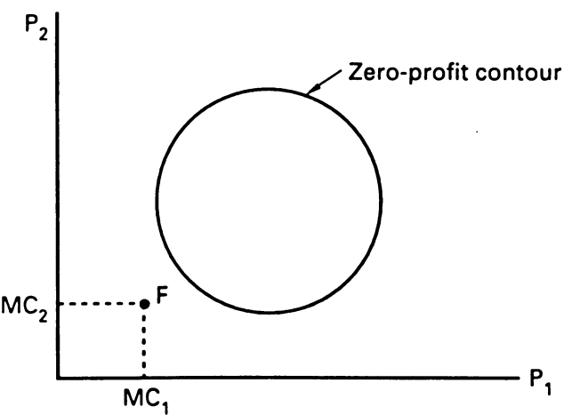
Figure 4.6 Zero-profit contour
