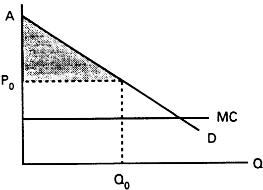
Figure 4.2 Consumer surplus
