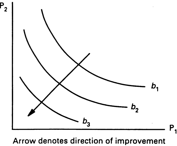
Figure 4.8 Isobenefit contours
