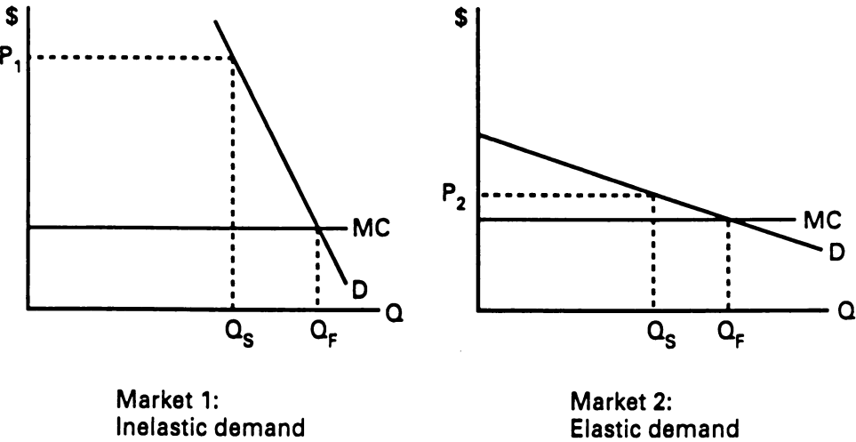
Figure 4.4 Ramsey prices
