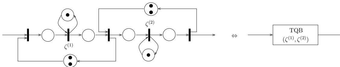
Figure 1: Tandem queues with blocking.
