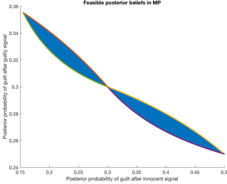
Figure 13: F(\Sigma, \pi) : an Illustration.
