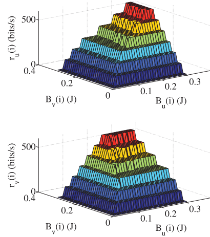
Fig. 12. Optimal communication rates r_u(i) (top) and r_v(i) (bottom) corresponding to different energy storage states, obtained by solving the LSPD problem.
