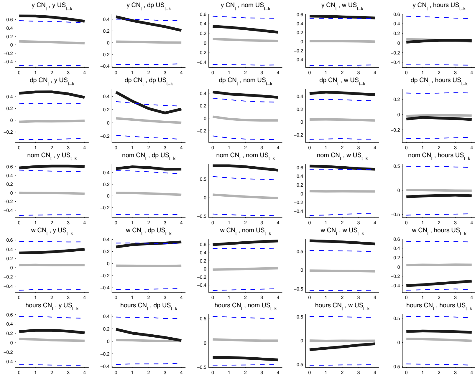
Figure 1: Data and model implied cross-correlations Canada–U.S. Data (dark), DSGE median (grey) and [ 5, 95] posterior bands (dashed)
