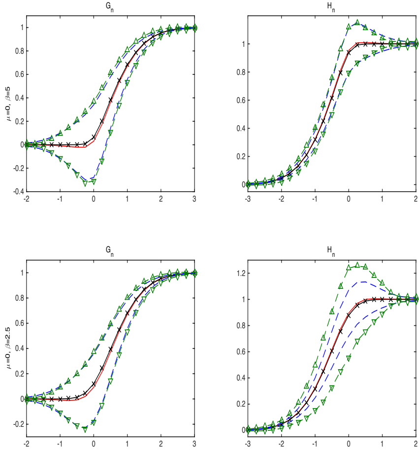
Figure 1. Simulation results for G_n (left) and H_n (right) for design \mu = 0, \beta = 5 (top) and design \mu = 0, \beta = 2.5 (bottom). Each plot contains the mean of the point estimator (solid red line) and the mean of the estimated 95% confidence bands (dashed blue lines), along with the true curve (solid black line, marked x) and 95% confidence bands constructed using the Monte Carlo standard deviation (dashed green lines, upper band marked \triangle and lower band marked \nabla ).
