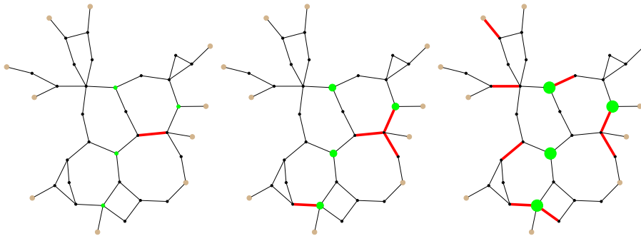
FIG. 3.4. 39-bus case with four wind farms (green dots; brown are generators, black are loads). Lines in red are at the maximum of \epsilon = .02 chance of exceeding their limit. The three cases shown are left to right .1%, 8%, and 30% average wind penetration. With penetration beyond 30% the problem becomes infeasible.
