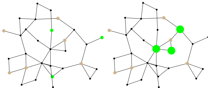
FIG. 3.5. 30-bus case with three wind farms. The case on the left supports only up to 10% penetration before becoming infeasible, while the one on the right is feasible for up to 55% penetration.
