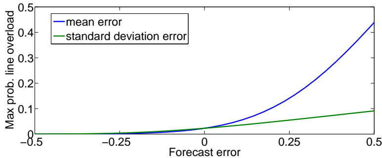
FIG. 3.7. BPA case solved with average penetration at 8% and standard deviations set to 30% of mean. The maximum probability of line overload desired is 2.27%, which is achieved with 0 forecast error on the graph. Actual wind power means are then scaled according to the x-axis and maximum probability of line overload is recalculated (blue). The same is then done for standard deviations (green).
