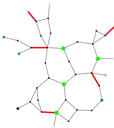
FIG. 3.3. 39-bus case. Red lines indicate high probability of flow exceeding the limit under the standard OPF solution. Generators are shades of blue, with darker shades indicating greater absolute difference between the chance-constrained solution and the standard solution.
