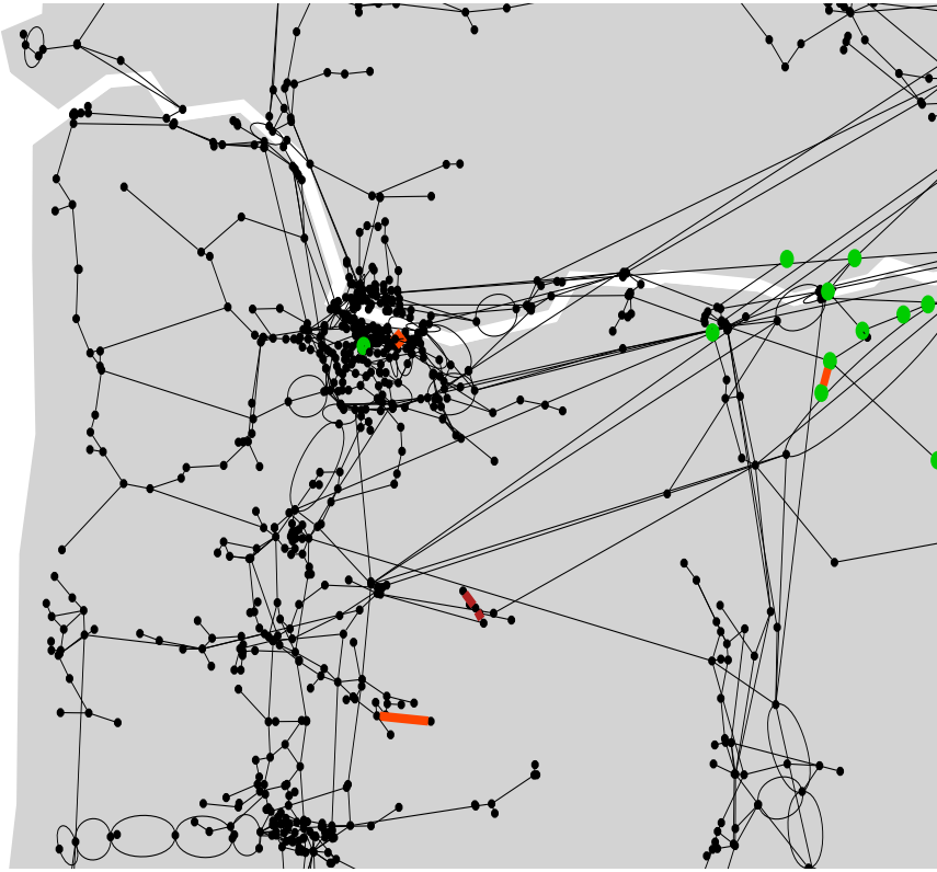
FIG. 0.1. Bonneville Power Administration [13] shown in outline under 9% wind penetration, where green dots mark actual wind farms. We set standard deviation to be 0.3 of the mean for each wind source. Our CC-OPF (with 1% of overload set as allowable) resolved the case successfully (no overloads) and was computed in seconds, while the standard OPF showed 8 overloaded lines, all marked in color. Lines shown orange are at 4% chance of overload. There are two dark red lines which are at 50% of the overload while other (dark orange) lines show values of overload around 10%.
