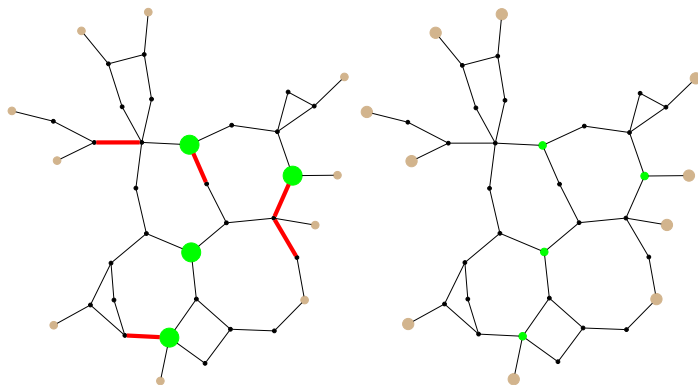
FIG. 3.2. 39-bus case under standard solution. Even with a 10% buffer on the line flow limits, five lines exceed their limit over 5% of the time with 30% penetration (left). The penetration must be decreased to 5% before the lines are relieved, but at great cost (right). The CC-OPF model is feasible for 30% penetration at a cost of 264,000. The standard solution at 5% penetration costs 1,275,020 – almost 5 times as much.
