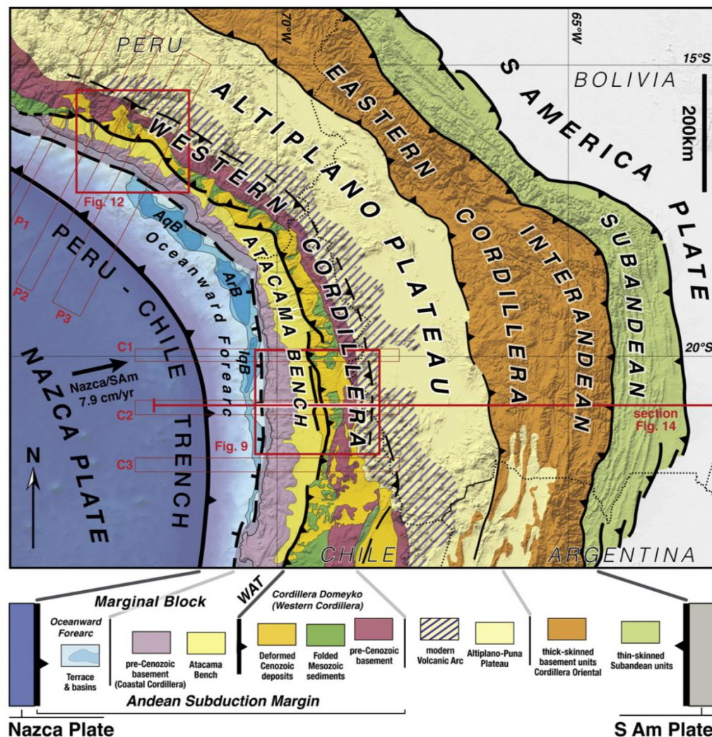
Figure 2. Geological sketch map of Andean orogen. The main morphological–structural units of the bivergent Central Andes (continental region with over-thickened crust constituting the core of the Andean orogen) are represented within horizontal boundary conditions (converging Nazca and South America plates) (Armijo et al., 2015).
