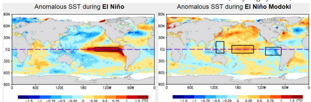
Figure 6—SST anomalies of eastern and central Pacific El Niño events (JAMSTEC)
