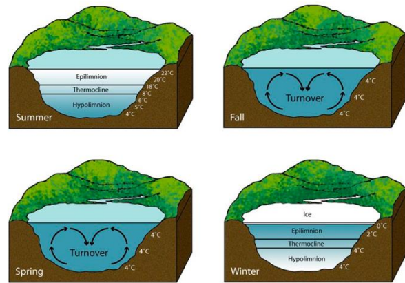
Figure 3: Cartoon illustrating a typical dimictic lake. While Titicaca is monomictic, these processes are similar (National Geographic)
