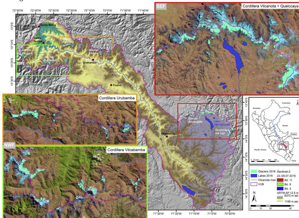
Figure 20. Overview of the Vilcanota-Urubamba-Picaduma catchment (VUB) situated in the central highlands of Peru (map) with main cities (red circles), prominent glaciers (turquoise triangles) and two principal reservoirs (Sibinacocha and Langui Loy). Glaciers belonging to the VUB (dashed pink delimitation) are highlighted as turquoise area. NWF=northwestern glacier fragment, SEF=southeastern glacier fragment. Reproduced from Drenkham et al., 2018.
