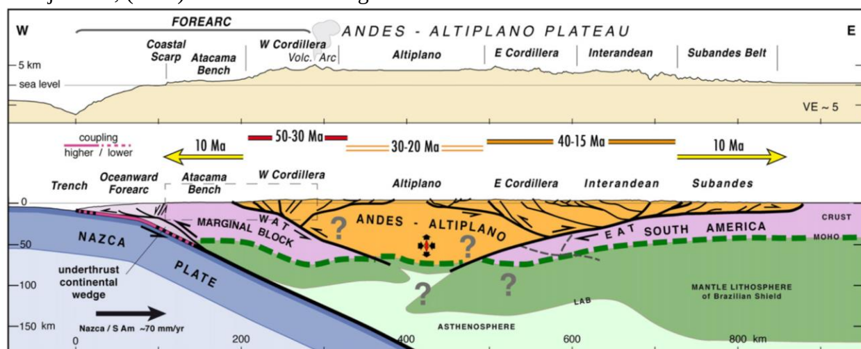
Figure 3. Large-scale 2D structure of Andean orogen. Interpreted section at 21°S, across the southern limb of the Andean orogen. (Armijo et al., 2015)
