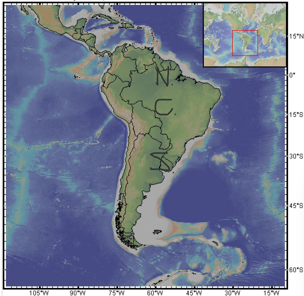
Figure 1. Topography map of South America featuring Andean mountains and country boundaries. From GeoMapApp (Ryan et al., 2009).
