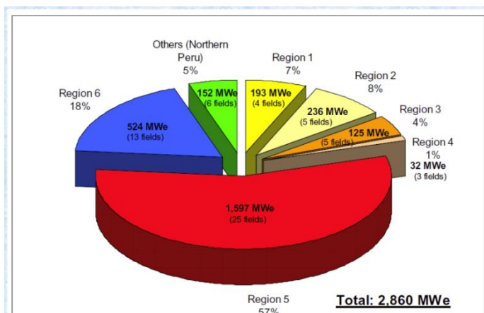
Figure 3: An estimate of potential energy output from geothermal harvesting. After Vargas and Cruz (2010).
