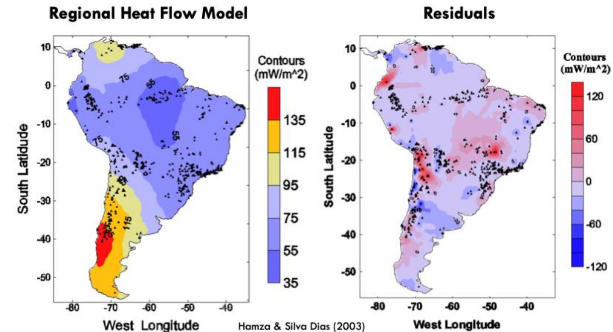
Figure 1: A sixth-degree polynomial fit to regional heat flow data in South America (left) with respective residuals (right). Locations of heat flow measurements marked with black triangles. After Hazma and Silva Dias (2003).
