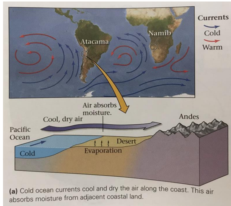
Figure 22 – Carton illustrating the formation of deserts along cold currents. From Marshak, 2015.
