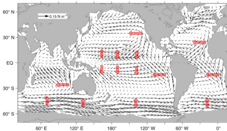
Figure 2. Vector field of global surface winds from the Encyclopedia of Atm. Sciences (2015), red arrows show major regions of surface current divergence leading to upwelling
