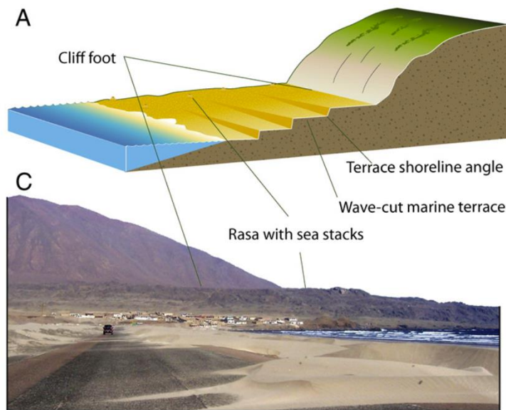
Figure 7: General sketch of a rasa, and a photo of the rasa with cliff and cliff base near Chala (Figure 2A and 2C in Regard et al., 2010)
