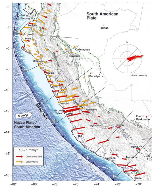
Figure 9: GPS velocity field expressed with respect to the SSA reference frame. [Villegas-Lanza et. al., 2016]
