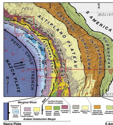
Figure 2: Map showing different tectonic/geological regions in the south of Peru [Armijo et al., 2015]
