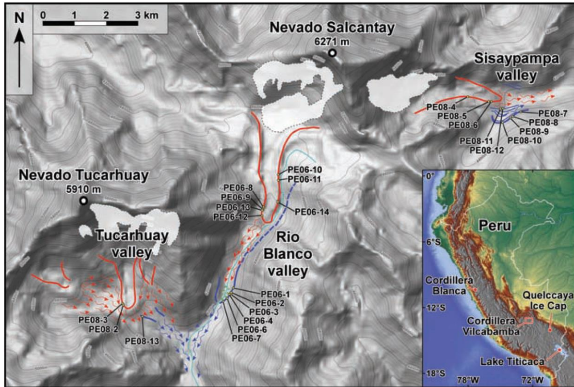
Figure 2: Geomorphic map of the area studied by Licciardi et al. (2009). Solid lines show inner (red) and outer (blue) moraines, and arrows show associated outwash; dashed lines indicate inferred locations. White areas represent approximate locations of present-day glaciers in mapped drainages. Base maps from Google Maps. Reproduced from Licciardi et al. (2006).
