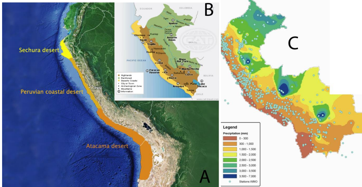
Figure 25 (A) Different deserts along the pacific coast of South America. (B) Different climate regions in Peru. Green, brown and yellow indicate rainforests, high lands and deserts coasts respectively. (C) Precipitation in Peru as indicated by the color bar.
