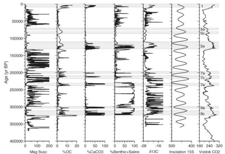
Figure 5: Multiproxy lake sediment record for the Titicaca basin showing glacial-interglacial cycles, with %organic carbon, %calcium carbonate, %Benthic+saline foraminifera, and \delta^{13}C increasing during interglacial periods (high Vostok CO_2 ), and magnetic susceptibility increasing during glacials (low Vostok CO_2 )(Fritz et al., 2012)
