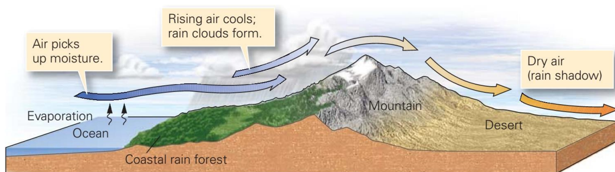
Figure 21 – Cartoon illustrating the formation of rain shadow deserts. From Marshak, 2015.
