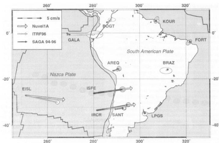
Figure 1: GPS data from four sites in the Nazca Plate (Easter Island, Galapagos, Robinson Crusoe and San Felix Islands) & from five sites in the stable core of the South American Plate used to calculate convergence rate [Angerman et. al., 1999]
