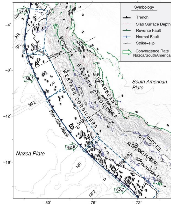
Figure 8: Neotectonic setting of the Peruvian margin showing focal mechanisms for M > 5 earthquakes [Villegas-Lanza et. al., 2016]
