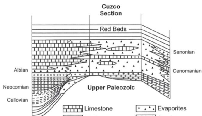
Figure 5: Generalized stratigraphy of the Cuzco area (Aral et al., 2011). The Yuncaypata Group consists of evaporites, limestones, and pelitic formations.
