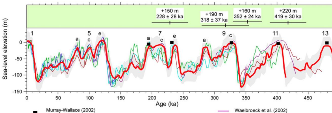
Figure 6: Correlation of marine terrace ages to marine isotopic stages (MIS) from the eustatic curve of Siddall et al. (2006 and references therein). +150, +160, +190, +220 m are names of the dated marine terraces of the San Juan de Marcona area and their respective age. (Figure 5 in Saillard et al., 2011)
