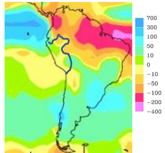
Figure 3—Precipitation anomaly (mm) during the average El Niño event (Dai and Wigley, 2000)
