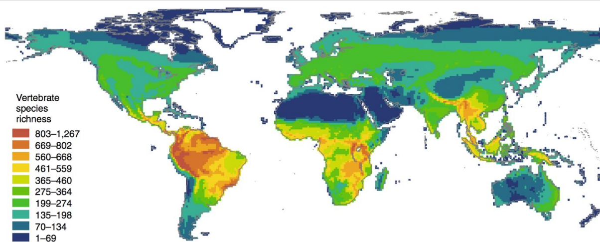
Figure 1. Global biodiversity of vertebrate species (amphibians, birds, and mammals) from a global database at 1° resolution (Antonelli et al., 2018).
