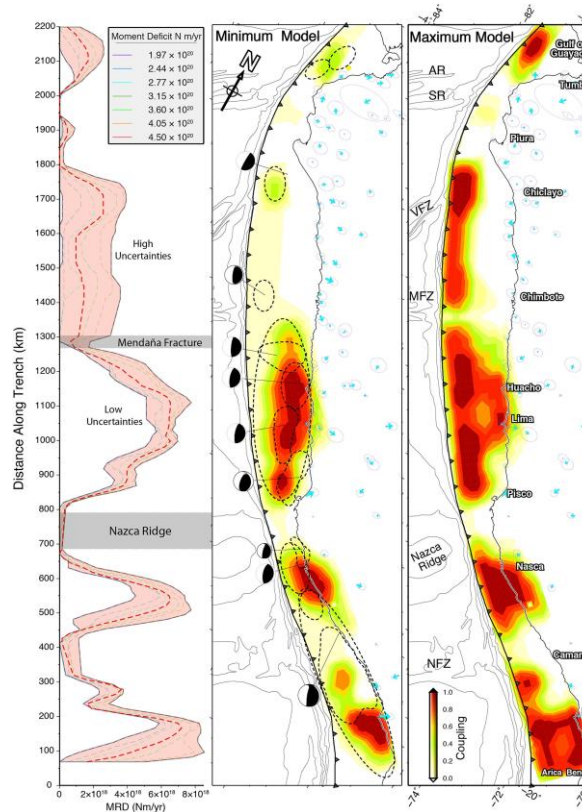
Figure 6: Inferred coupled regions of megathrust with estimated moment deficit (strain energy that has been built up during interseismic deformation) for different slip distribution models [Villegas-Lanza et. al., 2016]
