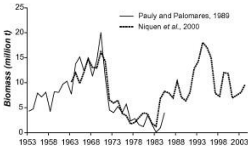
Figure 6 – A plot of anchovy biomass over time, as presented in Fréon et al 2008.
