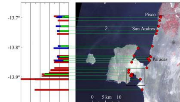
Figure 2: Measured tsunami heights and runup on a) Paracas Peninsula, from 2007 tsunami. Red bars indicate runup height. (Figure 2A in Fritz et al., 2008).
