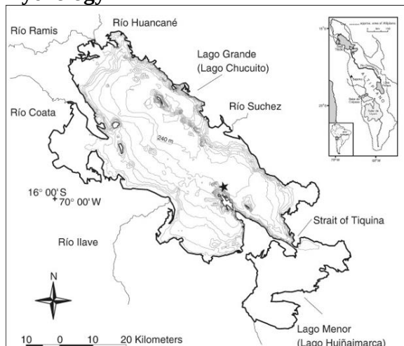
Figure 2: Hydrological map of Lake Titicaca (Fritz et al., 2007)
