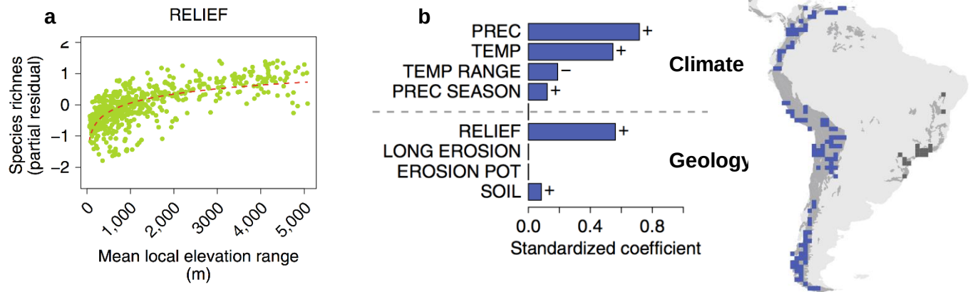
Figure 4. a) Global species richness variation with mean local elevation range (max-min elevation) showing a general increase with elevation range. b) Similar analysis for the Andes showing relief importance relative to climate parameters (Antonelli et al., 2018).
