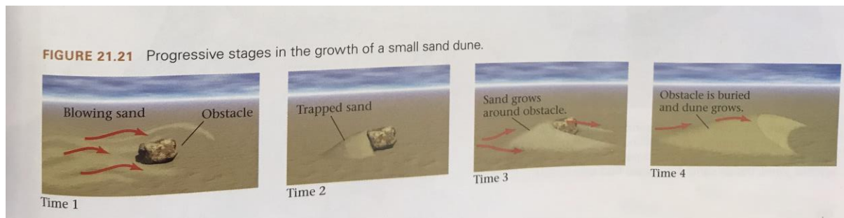
Figure 26 – A cartoon showing the formation of sand dunes.
