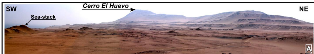
Figure 5: Panorama of the Cerro el Huevo marine terrace sequence in San Juan de Marcona (Figure 3A in Saillard et al., 2011)
