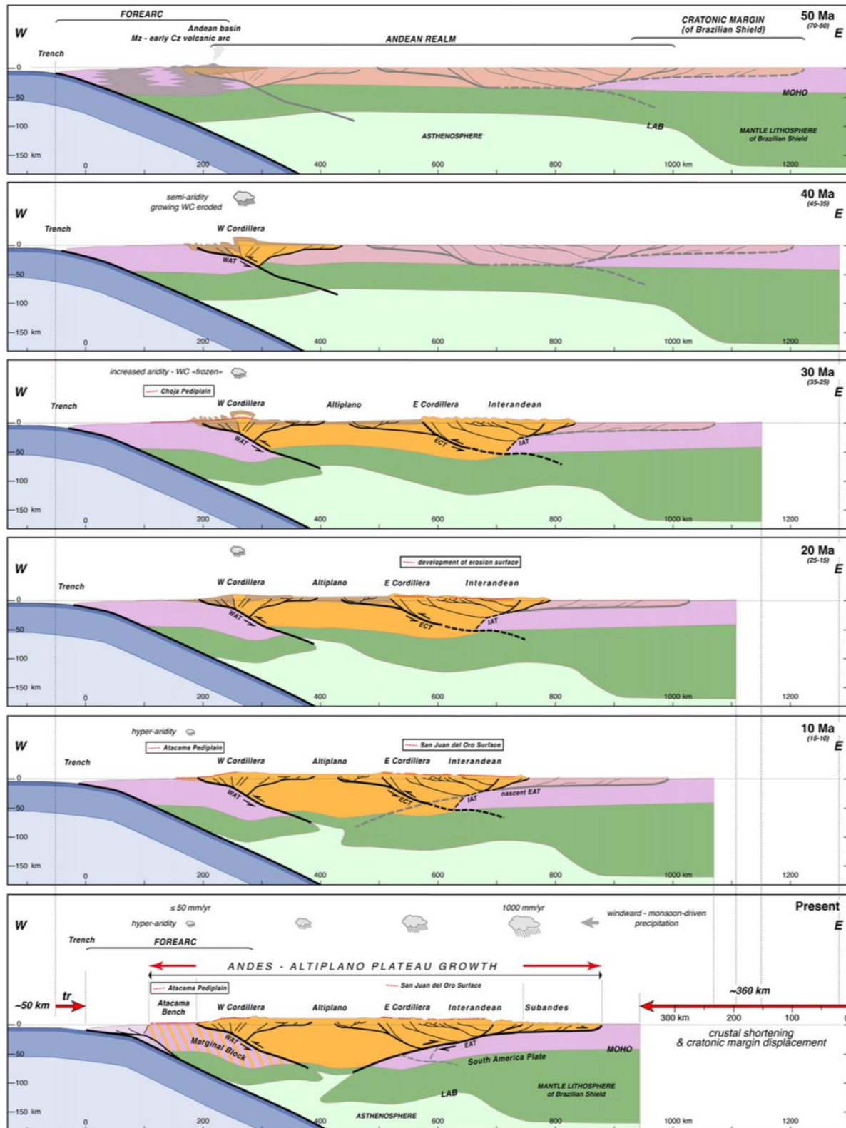
Figure 4. Evolution of Andean orogeny (from 50 Ma to present) (from Armijo et al., 2015). The growth process of the Central Andes is schematically represented for a section at 21°S, across the southern limb of the Andean orogen.
