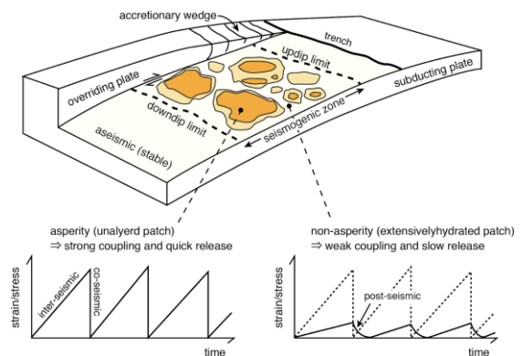
Figure 5: Diagram showing difference in behaviour of coupled (asperities) and uncoupled regions of the subduction zone megathrust
