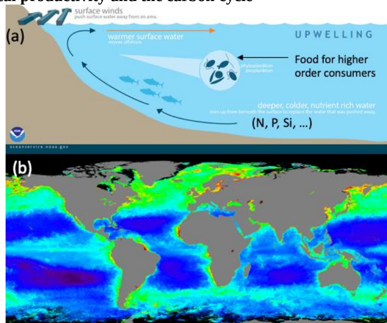
Figure 3. (a) Schematic diagram of the biological impact of upwelling from NOAA National Ocean Service, (b) satellite image of Chl-a concentration from the NASA Earth Observatory.
