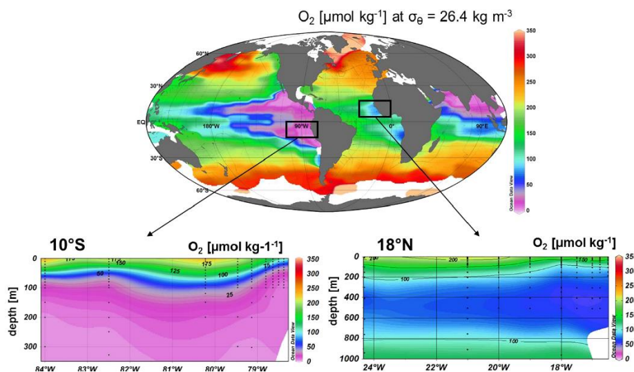
Figure 2 – Oxygen concentrations across the globe and in the oxygen minimum zones off the coast of South America and Northern Africa. From Löscher et al. 2015
