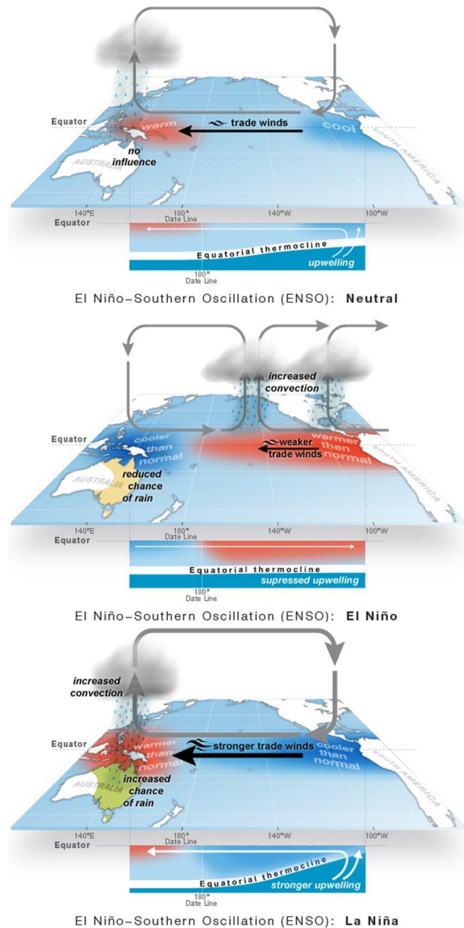
Figure 1—The three phases of ENSO (Bureau of Meteorology, 2008).
