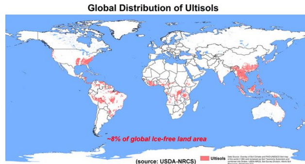
Figure 9: Map of global distribution of ultisols showing high prevalence in tropics/subtropics (USDA NRCS)
