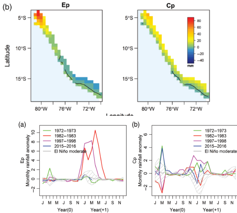
Figure 7—Top: Difference in spatial rainfall pattern during eastern Pacific (Ep) and central Pacific El Niño events. Bottom: Difference in temporal signature of eastern and central Pacific El Niño events (Sanabria et al., 2018)
