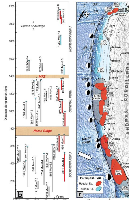
Figure 7: Recent major megathrust earthquakes and tsunamigenic earthquakes and their approximate slip distributions [Villegas-Lanza et. al., 2016]
