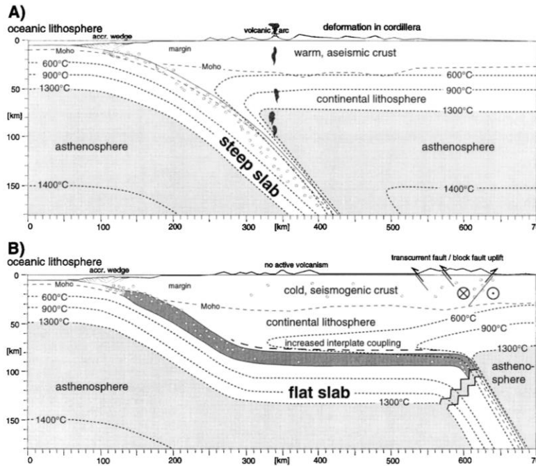
Figure 3: A - geometry and features of typical steep slab subduction. B - Geometry and features of flat slab subduction [Gutscher et al., 2000]
