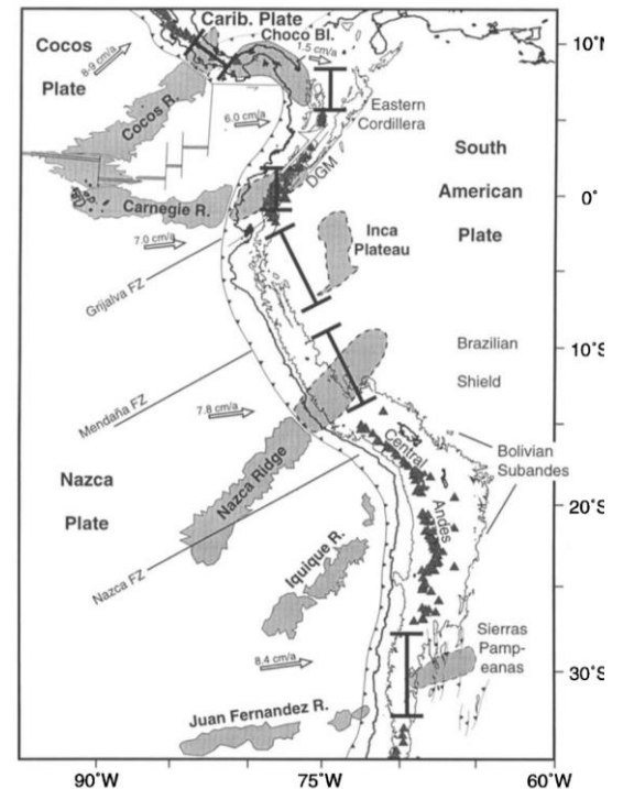
Figure 4: Tectonic setting of the Andean margin with flat slab segments indicated by thick brackets and subducting oceanic plateaus shaded gray [Gutscher et al., 2000]
