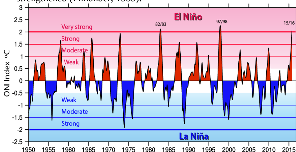
Figure 2—SST from Nino 3.4 region in the east Pacific where ENSO is monitored. An El Niño is classified as any three or more consecutive three-month periods (called the ONI index) when SST anomalies in the Nino 3.4 region exceed 0.5^{\circ}\text{C} (Trenberth et al., 2019)
