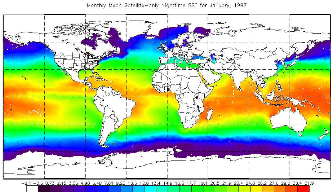
Figure 23 – Surface temperature of the oceans in January 1997 showing the cold Humboldt current.
