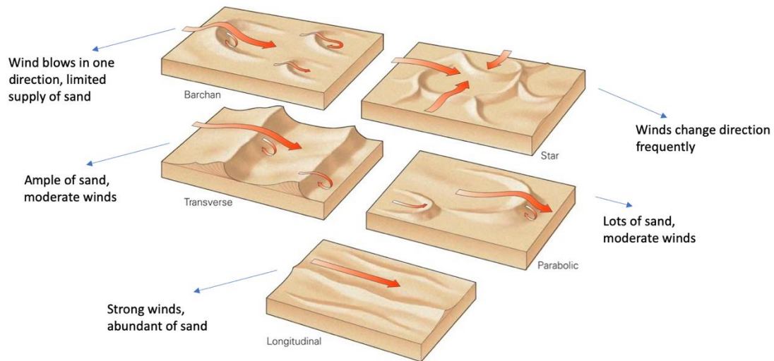
Figure 27 – An illustration showing different types of sand dunes and the conditions leading to their formation.
