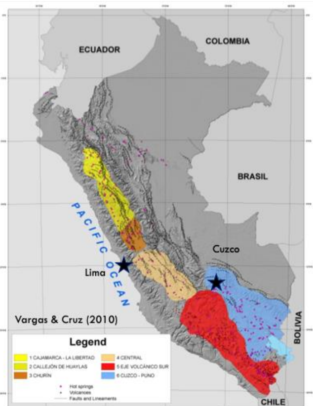
Figure 2: A map of Peru's six geothermal regions, with individual sites marked as pink dots. Eje Volcánico Sur (red) contains the most viable sites for geothermal energy harvesting. Modified after Vargas and Cruz (2010).
