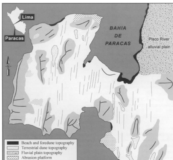
Figure 1: Geomorphology of Paracas Peninsula (Figure 2 in Psuty, 2005)
