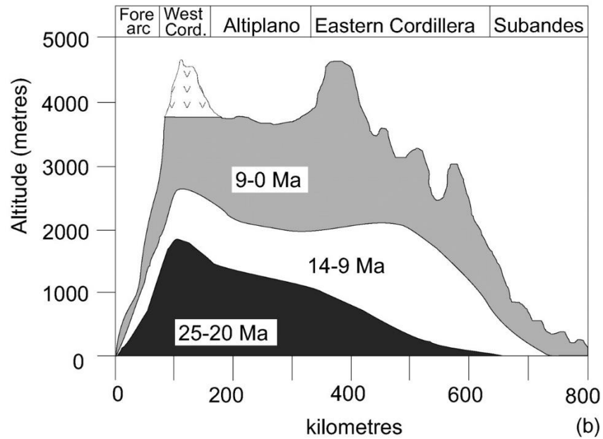
Figure 24 – Upper section: Estimated elevation through time for the Western Cordillera, Altiplano and Eastern Cordillera. Circles, diamonds and squares show data points from different sources. Lower section: Schematic west–east cross-section showing elevation at 18°S. From HARTLEY, 2007.
