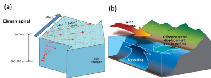
Figure 1. (a) Ekman spiral, (b)source: NOAA Fisheries
