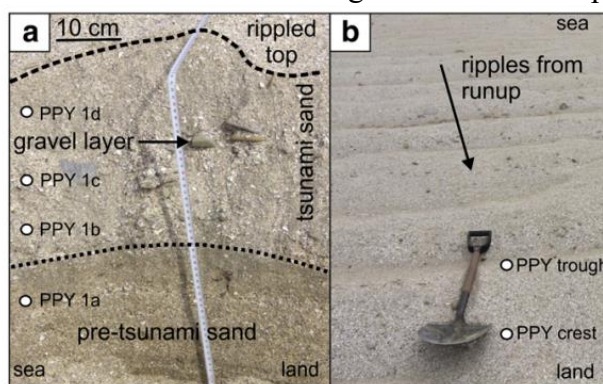
Fig. 8. Tsunami deposits (ca. 90 m from shoreline) and related grain size analysis at Playa Yumaque. a) Shelly tsunami sand with gravel layer and rippled top. b) Run-up ripples on
