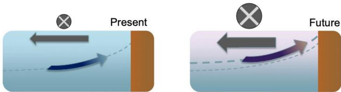
Figure 5. Schematic diagram depicting the relative projected change in wind strength (X), ocean temperature (colors), and location and magnitude of upwelling waters between the present (left panel) and future (right panel) as predicted by Oyarzún and Brierley et al., (2019)
