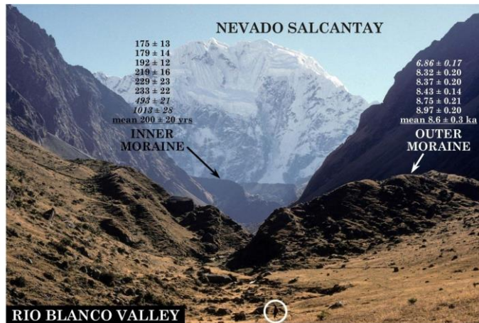
Figure 3: The view north towards Nevado Salcantay, showing the inner and outer moraines dated by Licciardi et al. (2008)
