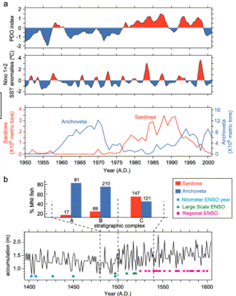
Figure 8 – Two different time series: Biomass of anchovies and sardines from 1950-2000 is paired with Pacific Decadal Oscillation (PDO), Sea surface temperature (SST) fluctuations. Biomass of sardines and anchovies from 1470-1540, interpreted from fish remains, is shown adjacent to a paleorecord of accumulation on the Quelccaya Ice Cap. (Sandweiss et al 2004)
