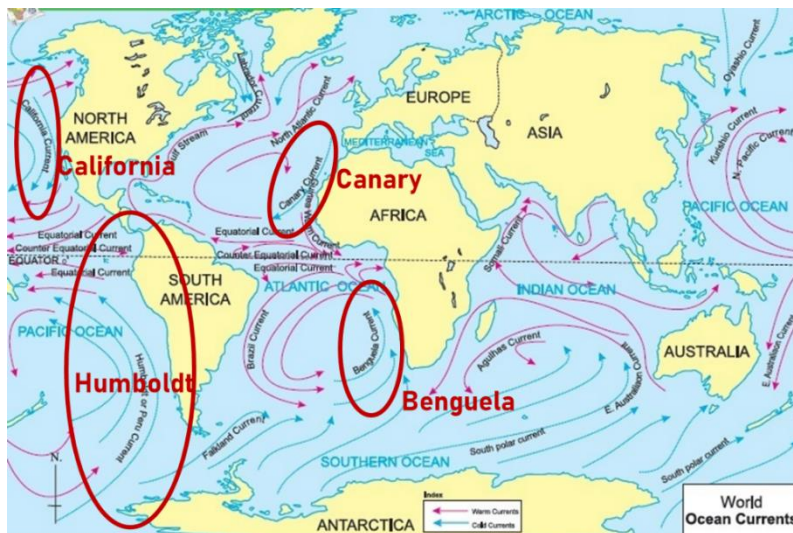
Figure 1 – Global map of major ocean currents with eastern boundary currents circled, adapted from Brainly.in.
