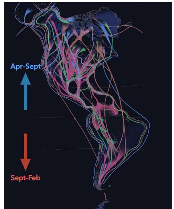
Figure 5. Schematic showing a range of avian flyways between North and South America (3).
