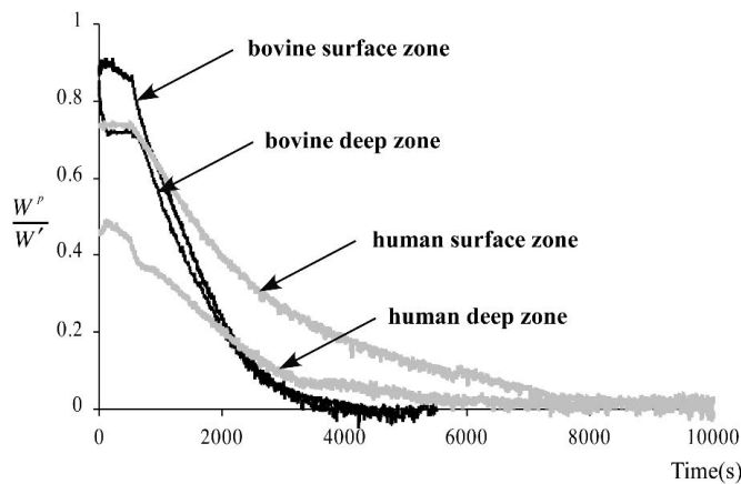
Fig 5. Experimental measurements of interstitial fluid load support ( W^p = load supported by fluid pressure, W = total applied load) in unconfined compression stress-relaxation of cylindrical disks of human and bovine cartilage are shown. The fluid load support is higher at the articular surface, where the ratio of tensile to compressive modulus is greatest. Reprinted with permission from Park S, Krishnan R, Nicoll SB, Ateshian GA: Cartilage interstitial fluid load support in unconfined compression. J Biomech 36:1785–1796, 2003.
