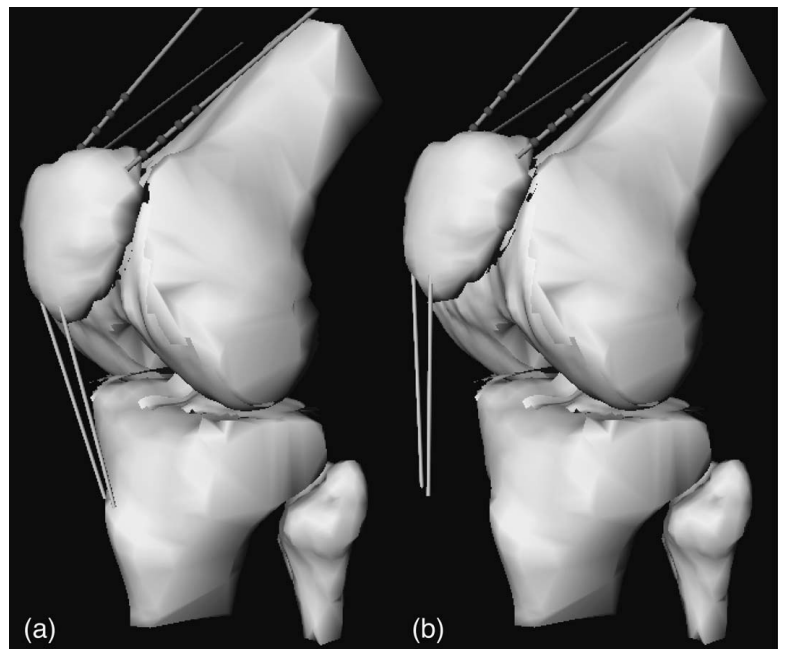
Fig 3A–B. A physics-based model of the knee of a patient with PFJ osteoarthritis. (A) The original model and (B) the model with simulated 20 mm of tuberosity transfer are shown. 24
