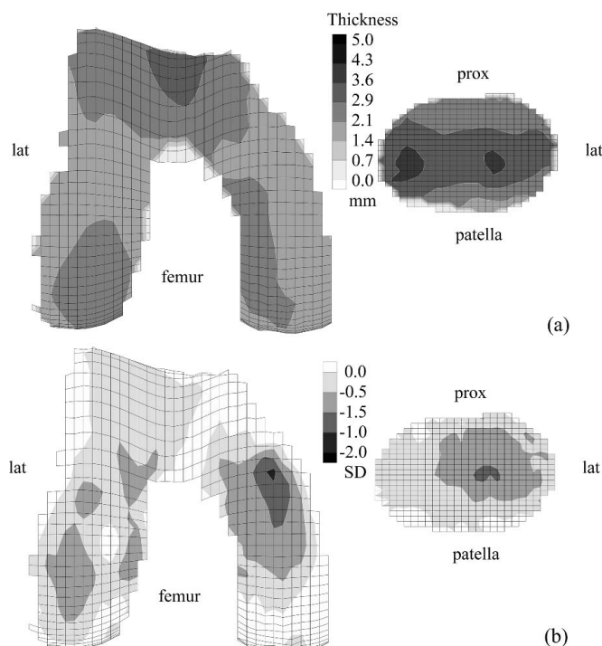
Fig 2A–B. Average cartilage thickness maps for the femoral and patellar surfaces of 33 knees with patellofemoral joint OA are shown. (A) The mean cartilage thickness map, plotted on mean articular surface topography of OA joints is shown. (B) The difference maps against the normal template, scaled by the local standard deviation of normal cartilage thickness, and plotted on the articular surface topography from the normal template are shown. Darker regions indicate regions of cartilage loss. Reprinted with permission from Cohen ZA, Mow VC, Henry JH, Levine WN, Ateshian GA: Templates of the cartilage layers of the patellofemoral joint and their use in the assessment of osteoarthritic cartilage damage. Osteoarthritis Cartilage 11:569–579, 2003.
