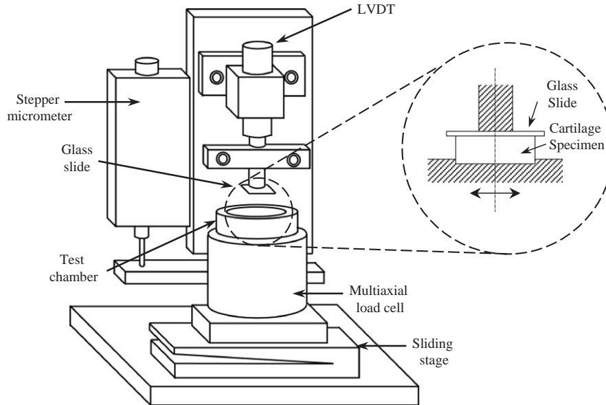
Fig. 1. Diagram of the friction testing device. The detail shows the orientation of the specimen relative to the glass slide and the sliding direction.
