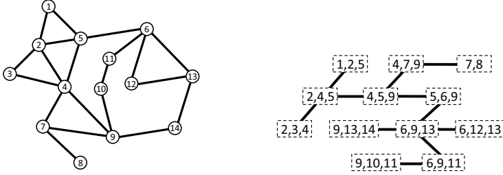
FIG. 8.1. The IEEE 14-bus test case (left figure) and its minimal tree decomposition (right figure)
