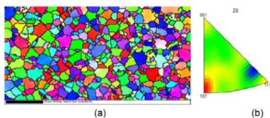
Fig. 8. (a) Representative EBSD map for normal direction of laser crystallized film with Euler angle coloring. Inverse pole figure (b) showing slight (110) texture normal to the film surface [7].
