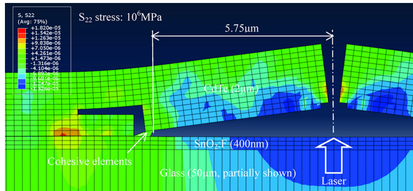
Fig. 15 S_{22} stress distribution of the region shown in Fig. 14 at the later stage (20 ns), showing some cohesive elements have been deleted. Deformation scale is 10× for viewing clarity.
