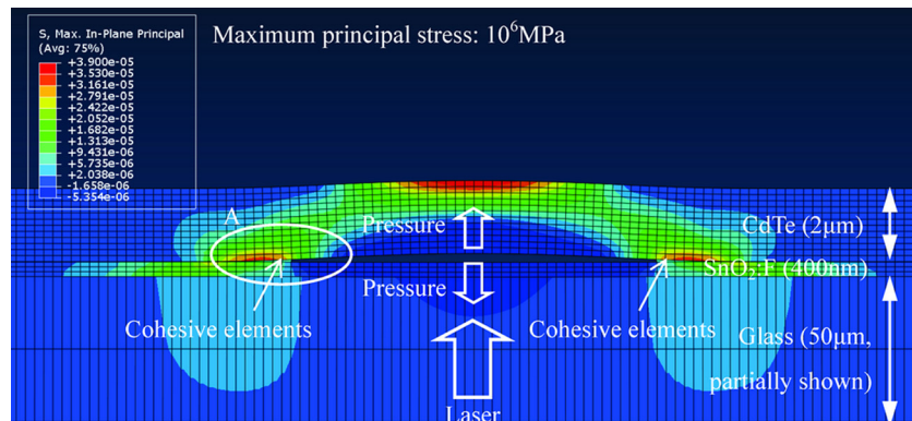
Fig. 13 Micro-explosion model with a pressure input at the CdTe/SnO 2 :F interface and the plasma dimension is 10 μm in width. A layer of cohesive elements is defined between the CdTe layer and SnO 2 :F layer. The CdTe film deforms due to the plasma expansion. The snapshot is taken at 10 ns. Deformation scale is 10× for viewing clarity.
