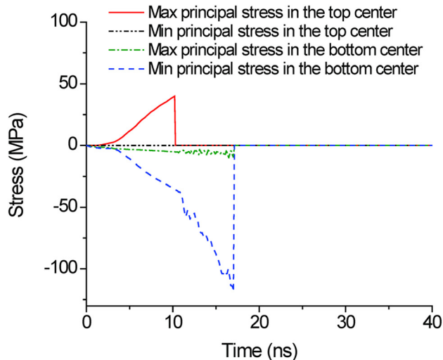
Fig. 16 Stress evolution of the failed elements at the top center and bottom center of the CdTe layer. Tensile stress occurs on the top, while compressive stress occurs at the bottom. The stresses drop to zero once the Coulomb-Mohr criterion is met.
