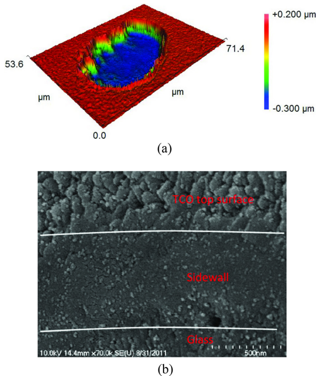
Fig. 9 (a) 3D scanning of the removal film profile by optical profilometry and (b) SEM image of the sidewall of film removal by single pulse processed \text{SnO}_2\text{:F} samples from film side at a fluence of 127 \text{ J/cm}^2
