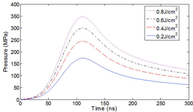
Fig. 12 Temporal distribution of the plasma pressure at different fluences from 0.2 J/cm 2 to 0.8 J/cm 2
