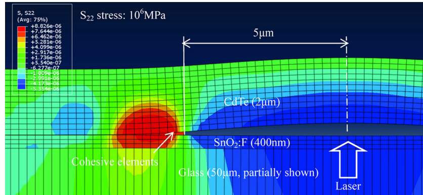
Fig. 14 S_{22} stress distribution of the magnified area A in Fig. 13 at the same moment. The cohesive elements have been deformed due to S_{22} stress. Deformation scale is 10× for viewing clarity.
