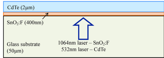
Fig. 1 Illustration of the glass-side laser scribing model for SnO 2 :F and CdTe film removal. Lasers with wavelength of 1064 nm and 532 nm are adopted for SnO 2 :F and CdTe scribing, respectively.
