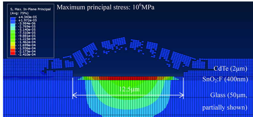
Fig. 18 Maximum principal stress distribution at 66 ns. The film has been completely removed with an opening width of 12.5\mu\text{m} . Both brittle failure and film delamination contribute to the film removal. Deformation scale is 2\times for viewing clarity.
