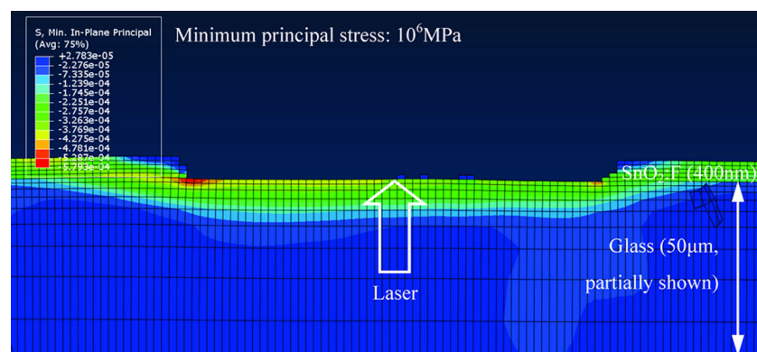
Fig. 5 The result of \text{SnO}_2\text{:F} removal by 3 \text{ J/cm}^2 laser irradiation based on the fully coupled thermal stress analysis. An 8.3 \mu\text{m} opening is generated. The snapshot is taken at 200 ns. Deformation scale is 10\times for viewing clarity.
