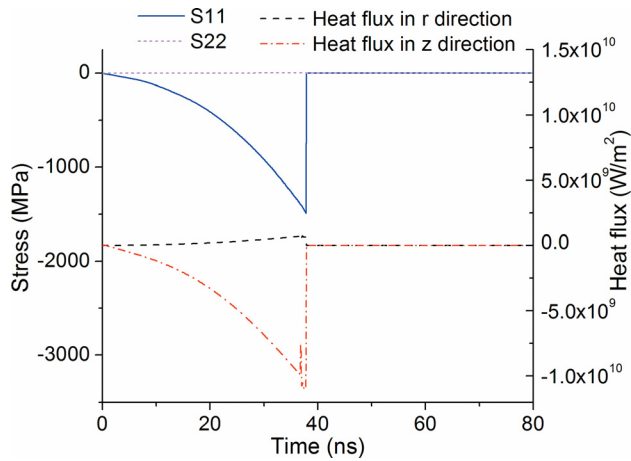
Fig. 4 Principal stress and heat flux history in an element at \text{SnO}_2\text{:F} film center. The element deletion occurs at 38 ns. Heat flux drops to zero due to instantaneous dependence between thermal and mechanical analyses.
