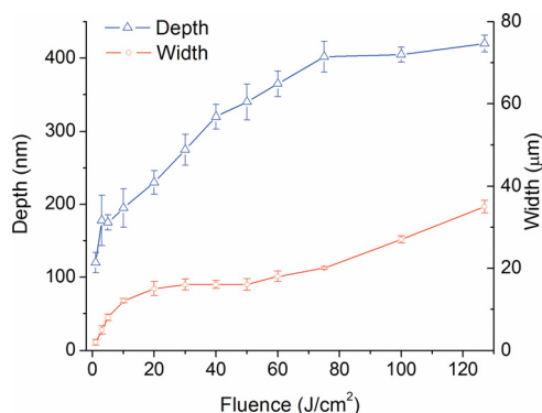
Fig. 10 Dependence of removal depth and width on laser fluence. Error bars indicate standard deviation.
