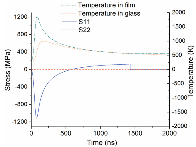
Fig. 6 Temperature and stress history in a deleted element at \text{SnO}_2\text{:F} film center treated at a fluence of 1 \text{ J/cm}^2 . The element is subjected to a compressive stress followed by a tensile stress. The element fails when the tensile failure stress is met at 1430 ns.
