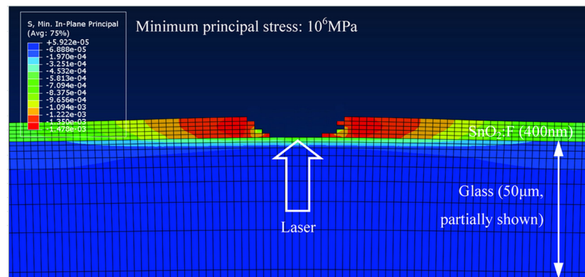
Fig. 3 Fully coupled thermal stress analysis of SnO 2 :F removal by laser irradiation at a fluence of 3 J/cm 2 at 38 ns. Absorption of laser energy induces local thermal expansion and thermal stress. Elements experiencing a principal stresses larger than the failure strength are deleted from calculation. A 2 μm opening has been generated accordingly. 10× Deformation scale for viewing clarity.
