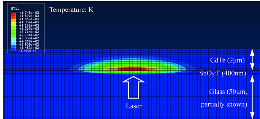
Fig. 11 Temperature distribution of CdTe/SnO 2 :F/glass multilayer system under laser irradiation at a fluence of 0.2 J/cm 2
