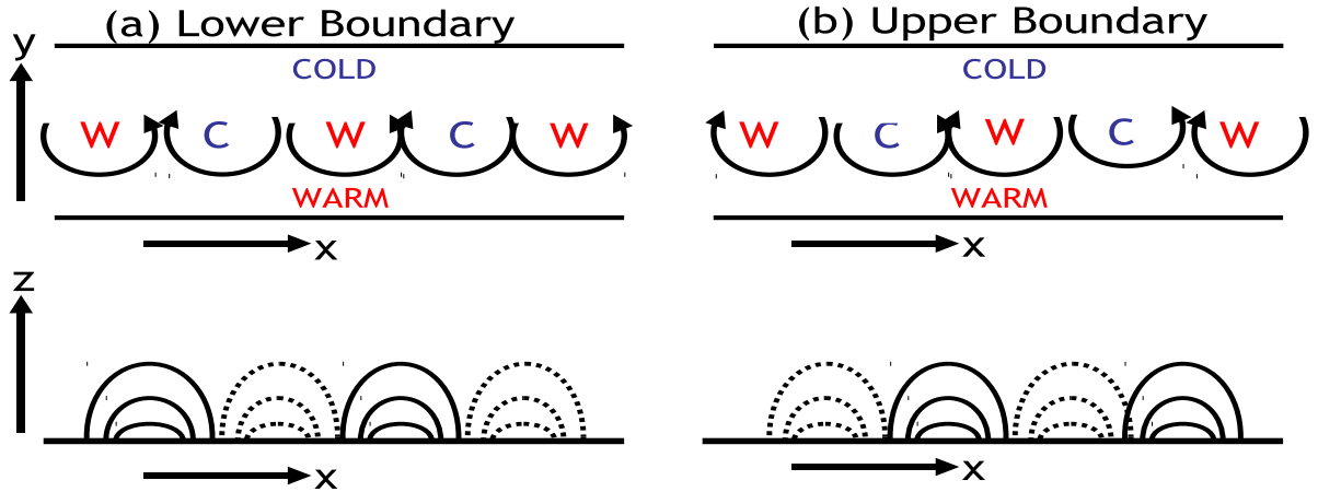
Figure 4: Illustration of the circulation associated with the temperature anomalies on (a) the lower and (b) the upper boundaries. These temperature anomalies would be induced by a meridional displacement of air parcels on the boundaries. The lower panel shows the vertical profile of meridional velocity associated with the temperature anomalies. The solid lines indicate velocity in the positive y direction and the dotted indicated velocity in the negative y direction.
