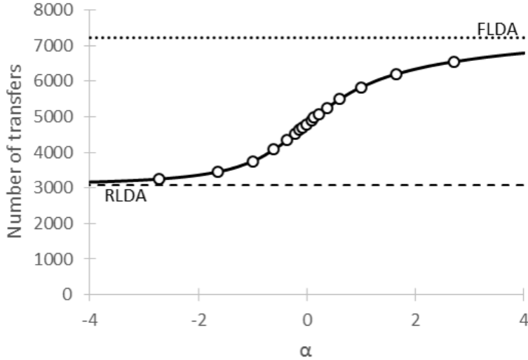
Figure 4: Number of reassigned students versus \alpha . The number of reassignments under the extreme values of \alpha , namely, \alpha = \infty (FLDA) and \alpha = -\infty (RLDA) are shown via dotted lines.
