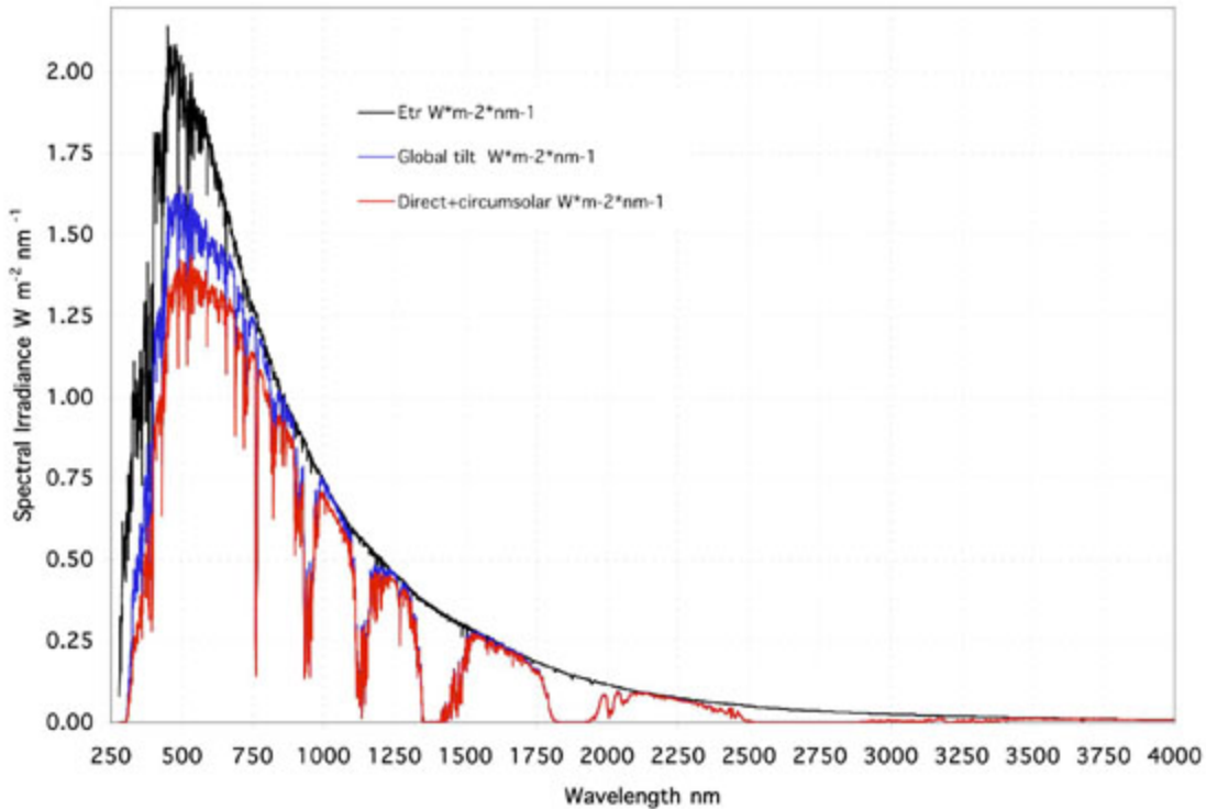
ASTM G173-03 Reference Spectra
