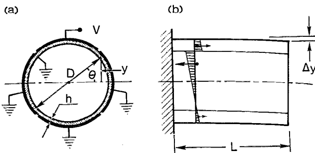
FIG. 2. Deflection of a tube scanner in the unipolar arrangement. (a) A voltage is applied on only one quadrant of the outer metal coating. All other quadrants and the inner metal coating are grounded. (b) At equilibrium, a distribution of stress and strain is established such that the total force and torque at each cross section is zero. This condition determines the y displacement.
