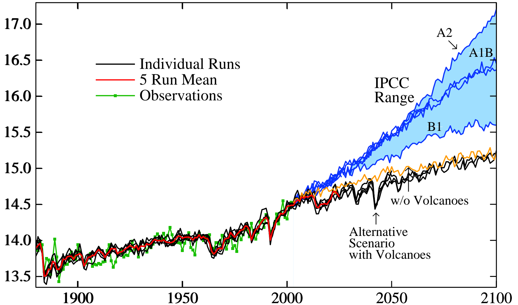
Figure 21. Global surface temperature simulations extended through 21 st century (reference 5).
