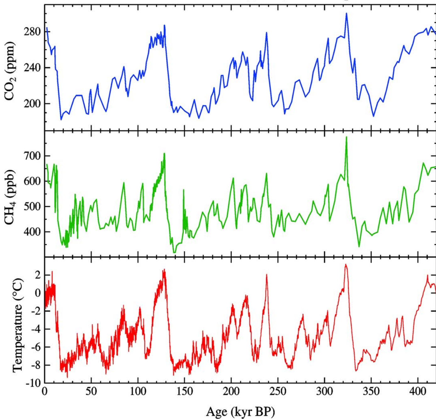
Figure 9. Vostok carbon dioxide, methane, and temperature record for the past 400,000 years (reference 3).
