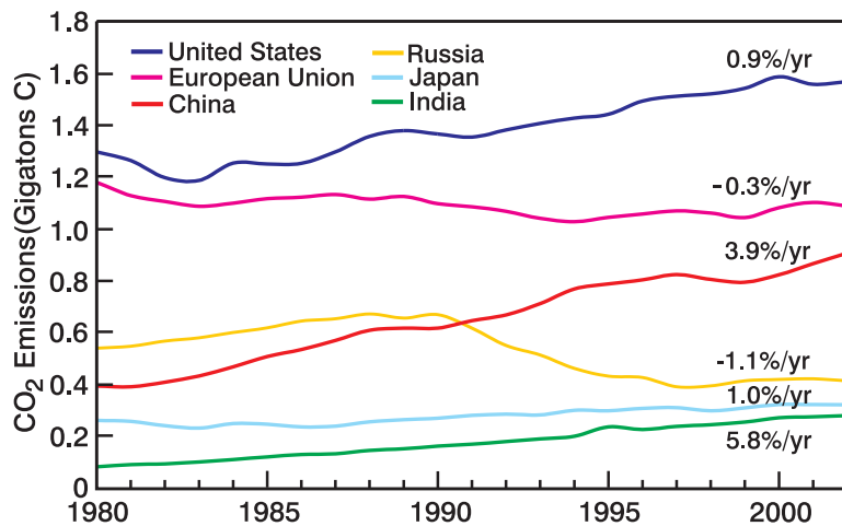
Figure 24. World energy consumption (top) and world CO 2 emissions (bottom) based on data from EIA (13). Pie charts are the division of energy use and CO 2 emissions among countries in 2002. Line graphs show the histories since 1980 including the annual growth rates.
