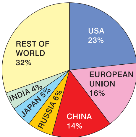
Figure 24. World energy consumption (top) and world CO 2 emissions (bottom) based on data from EIA (13). Pie charts are the division of energy use and CO 2 emissions among countries in 2002. Line graphs show the histories since 1980 including the annual growth rates.
