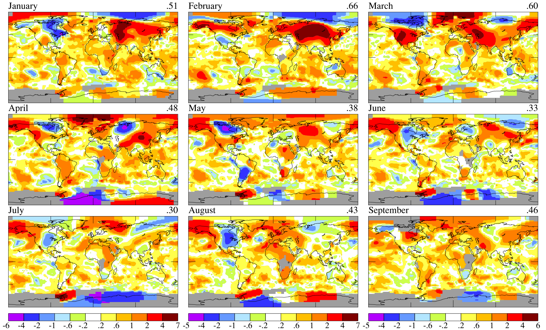
Figure 4. Temperature anomalies in 2004, relative to 1951-1980 mean (reference 1).
