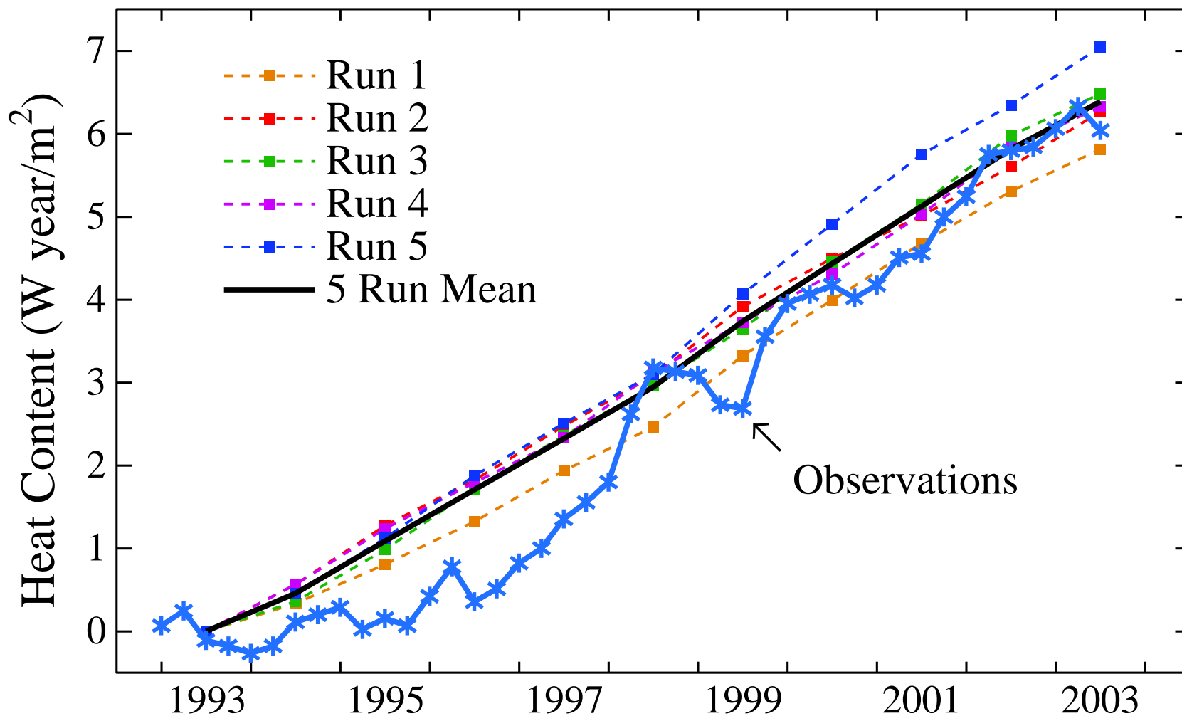
Figure 14. Ocean heat content change between 1993 and 2003 in top 750 meters of the world ocean. Observations from reference 11. Climate model the same as in previous two figures, driven by climate forcings in Figure 11.
