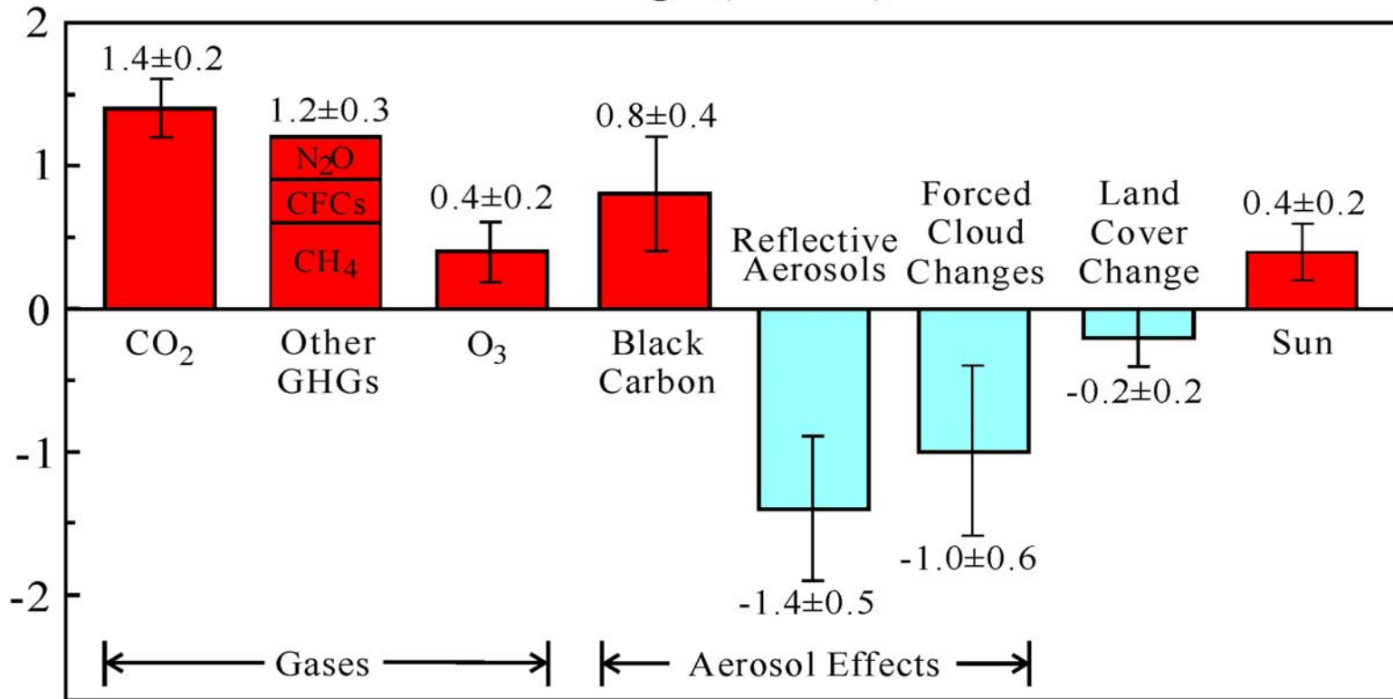
Figure 6. Climate forcing agents in the Industrial Era (reference 2). A climate forcing is a mechanism that alters the global energy balance. A forcing can be natural – fluctuations in the sun’s brightness, for example – or human made, such as aerosols and greenhouse gases. Human-made climate forcings now dominate natural forcings.
