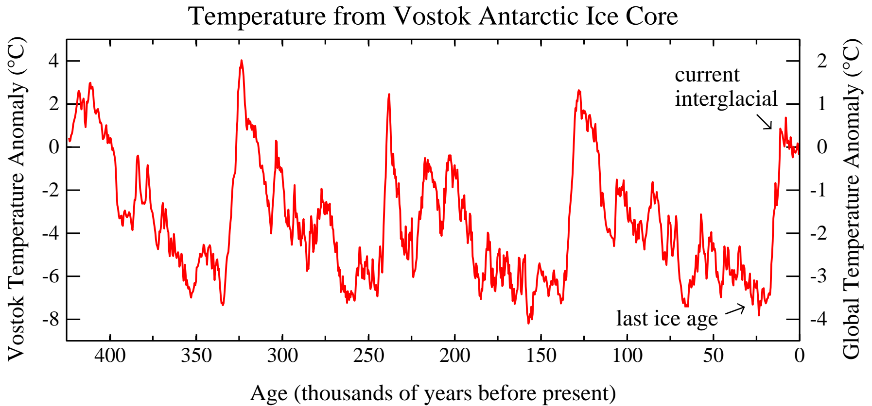
Figure 8. Vostok (Russian base in central Antarctica) temperature for past 400,000 years (reference 3).
