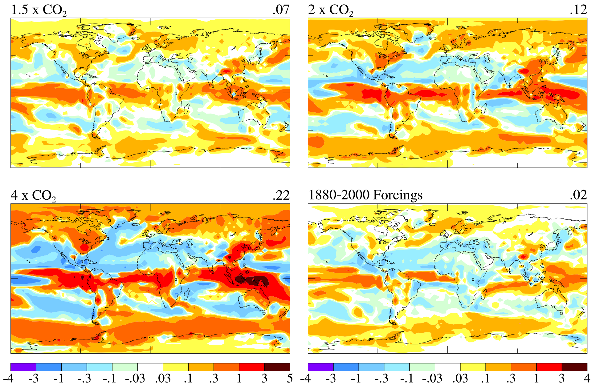
Figure 19. Precipitation changes with increasing CO 2 and "all forcings" in 2000 (reference 7).
