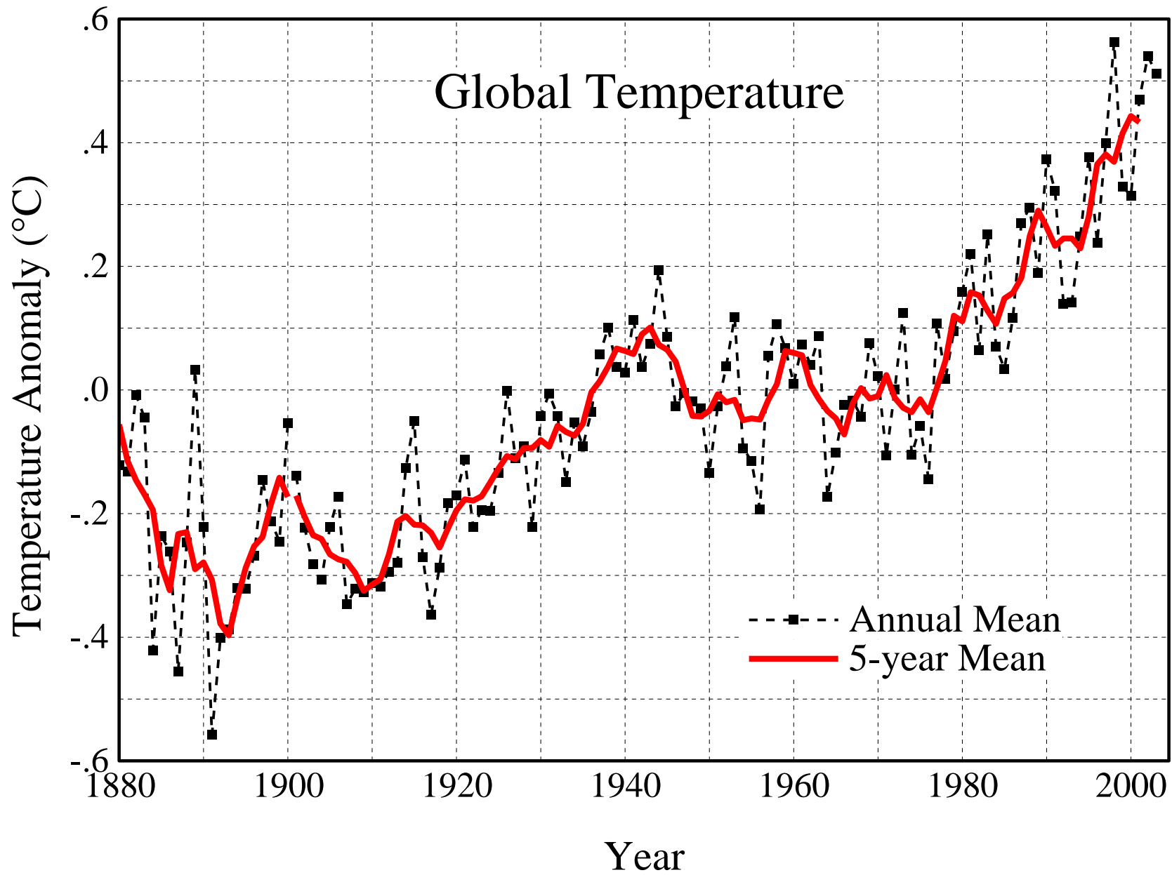
Figure 5. Global mean temperature change, based on meteorological stations before 1900 and stations plus sea surface temperatures after 1900 (reference 1).
