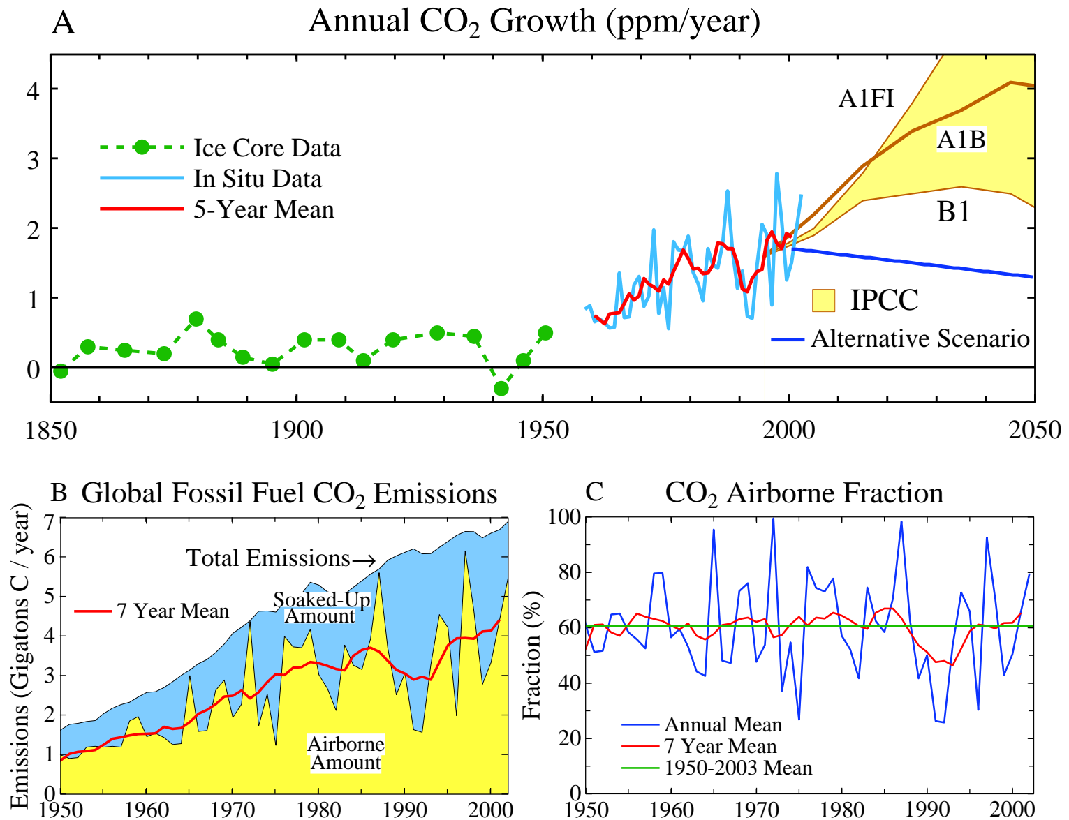
Figure 22. (A) Annual growth of atmospheric CO 2 based on measurements through 2003 and on scenarios of IPCC (reference 8) and Hansen and Sato (reference 9). Fossil fuel emissions are continuing to grow as shown by the top curve in (B). The average fraction of emissions that remains airborne (C) continues to be about 60%, implying that the underlying CO 2 growth rate is now 1.9 ppm/year, closer to the IPCC (2001) scenarios than to the "Alternative Scenario" (reference 10).
