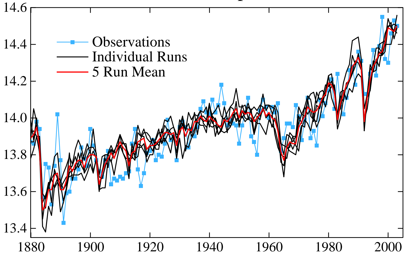
Figure 12. Observed and simulated global surface temperature change for forcings of Figure 11. The five model runs differ in initial ocean and atmosphere conditions, and thus follow their own chaotic paths (reference 5).
