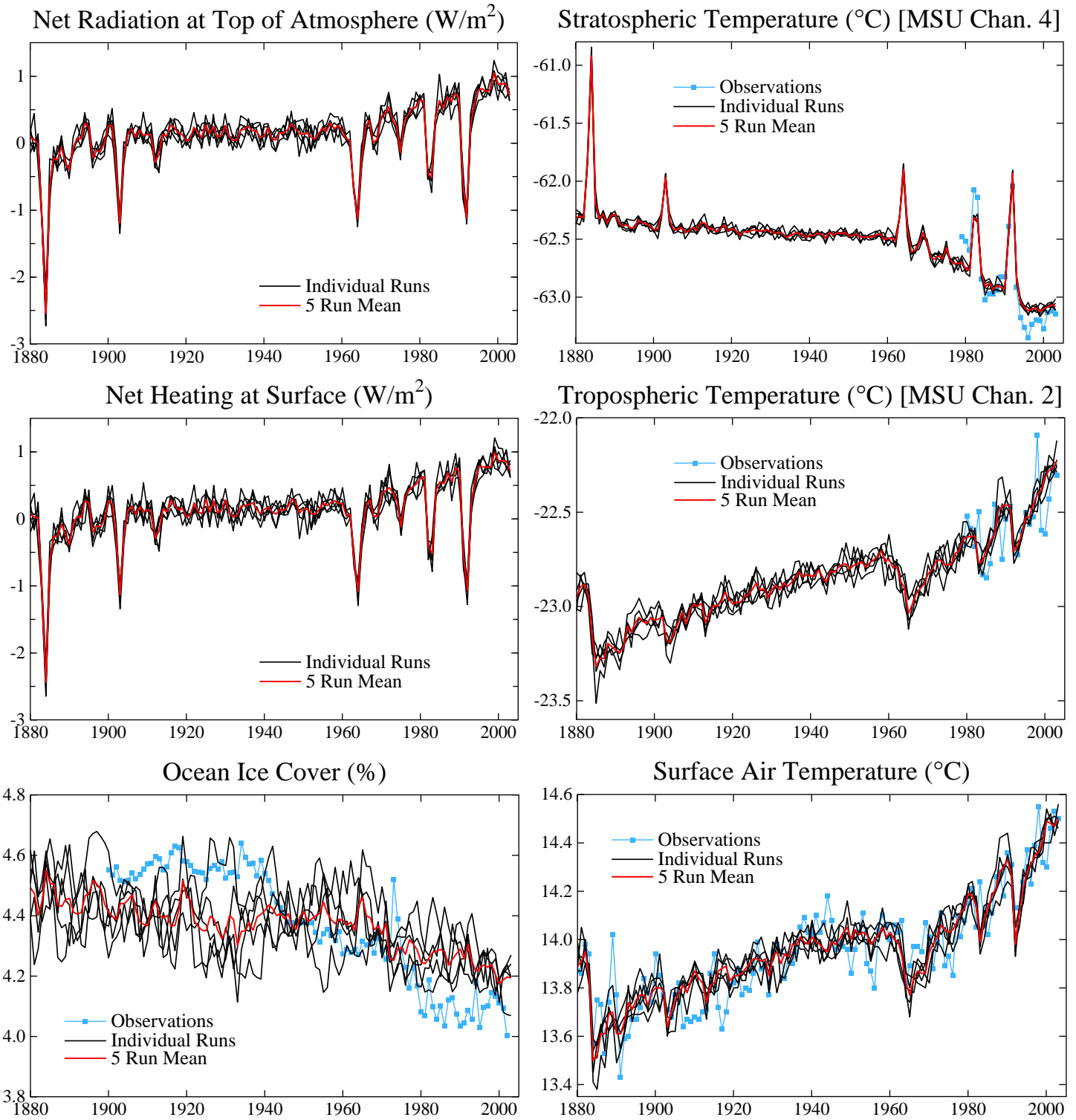
Figure 13. Global climate simulations driven by forcings of Figure 11 (reference 5).
