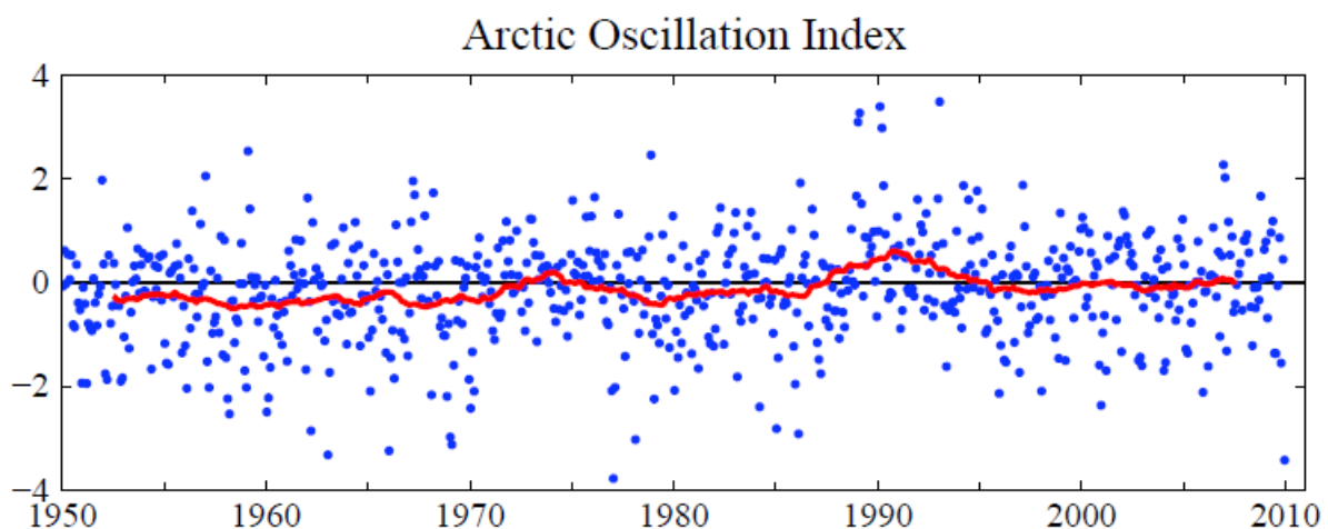
Figure 8. Arctic Oscillation (AO) Index. Negative values of the AO index indicate high pressure in the polar region and thus a tendency for weak zonal winds that facilitate cold air outbreaks to middle latitudes. Blue dots are monthly means and the red curve is the 60-month (5-year) running mean.
