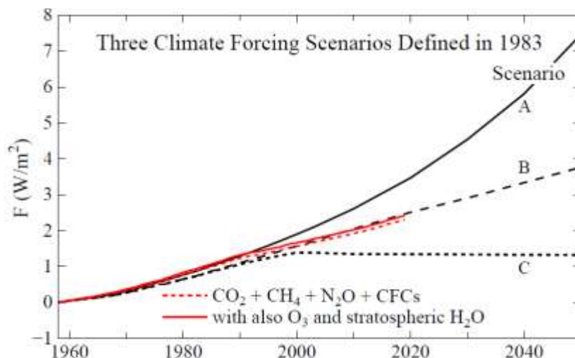
Fig. 30.2. Greenhouse gas climate forcing for three scenarios and for the real world (red).
