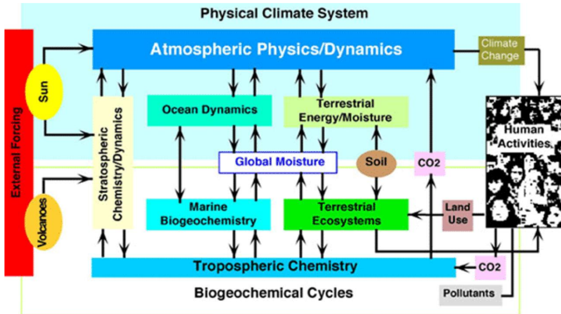
Fig. 32.1. Simplified Bretherton Wiring Diagram.
