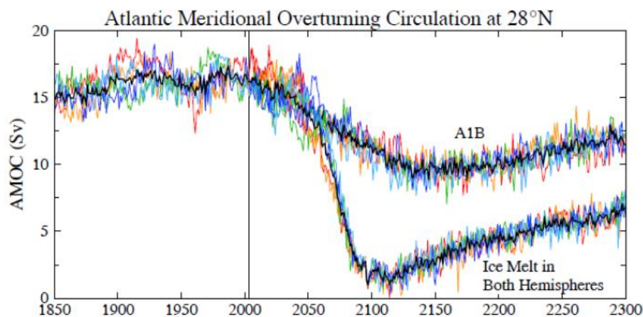
Foreword Figure 5. AMOC strength at 28°N in five simulations and their mean (black line) for IPCC A1B scenario and ice melt in both hemispheres, two-thirds of it from Antarctica.
