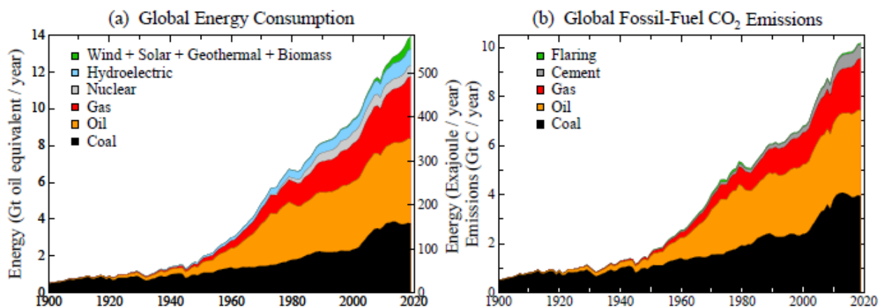
Foreword Figure 1. Global energy consumption (a) and fossil fuel CO 2 emissions (b) from 1900 through 2019.
