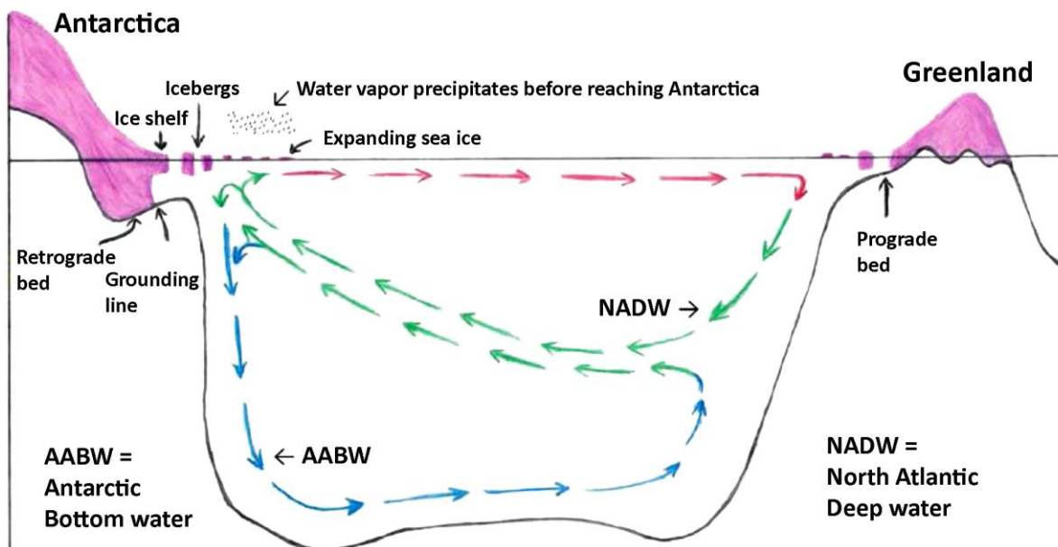
Foreword Figure 2. Schematic diagram of the surface origin of two water masses that fill most of the world ocean: North Atlantic Deep Water (NADW) and Antarctic Bottom Water (AABW). The upper circulation cell is the Atlantic Meridional Overturning Circulation (AMOC) and the deeper circulation is the Southern Meridional Overturning Circulation (SMOC). Physical processes occurring near the ice sheets are discussed later in this preface and further by Hansen et al. (2016).
