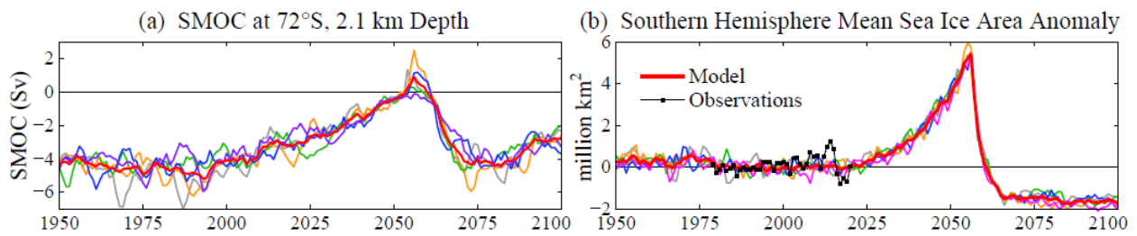
Foreword Figure 4. (a) SMOC mean circulation at 72°S (excludes eddy-induced transport), and (b) annual sea ice area anomaly ( 10^6 \text{ km}^2 ) relative to 1979-2000 in five model runs and observations. One Sverdrup (Sv) is 10^6 \text{ m}^3/\text{s} or \sim 3 \times 10^4 \text{ Gt}/\text{year} . A Gt is a billion tons.
