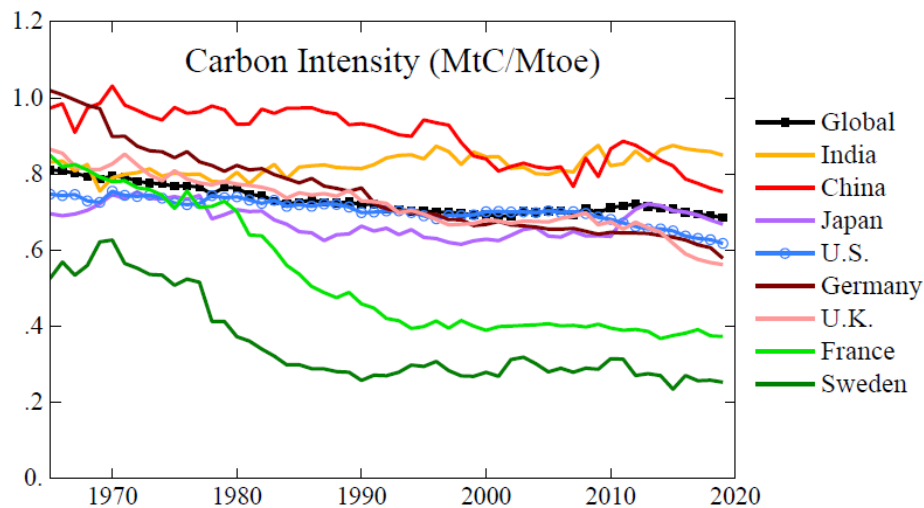
Foreword Figure 7. Carbon intensity (carbon per unit energy) of global and national energies. MtC is megatons of carbon. Mtoe is megatons of oil equivalent.
