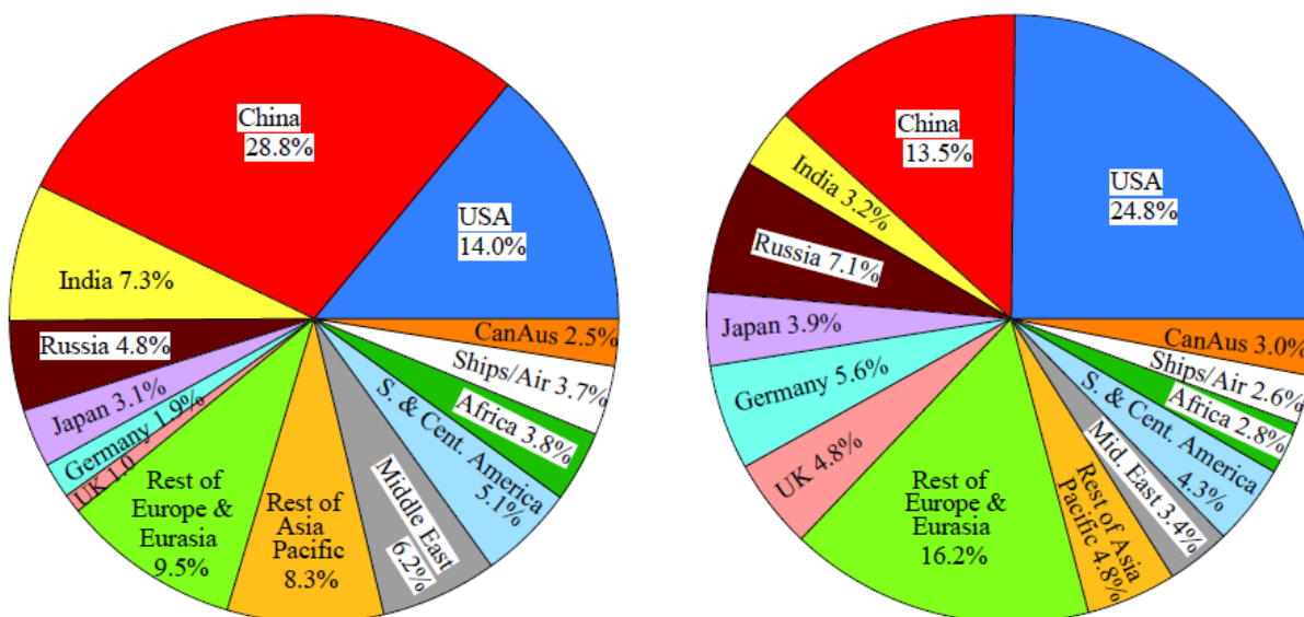
Foreword Figure 6. Fossil fuel emissions in 2018 (left) and cumulative 1751-2018 emissions.
