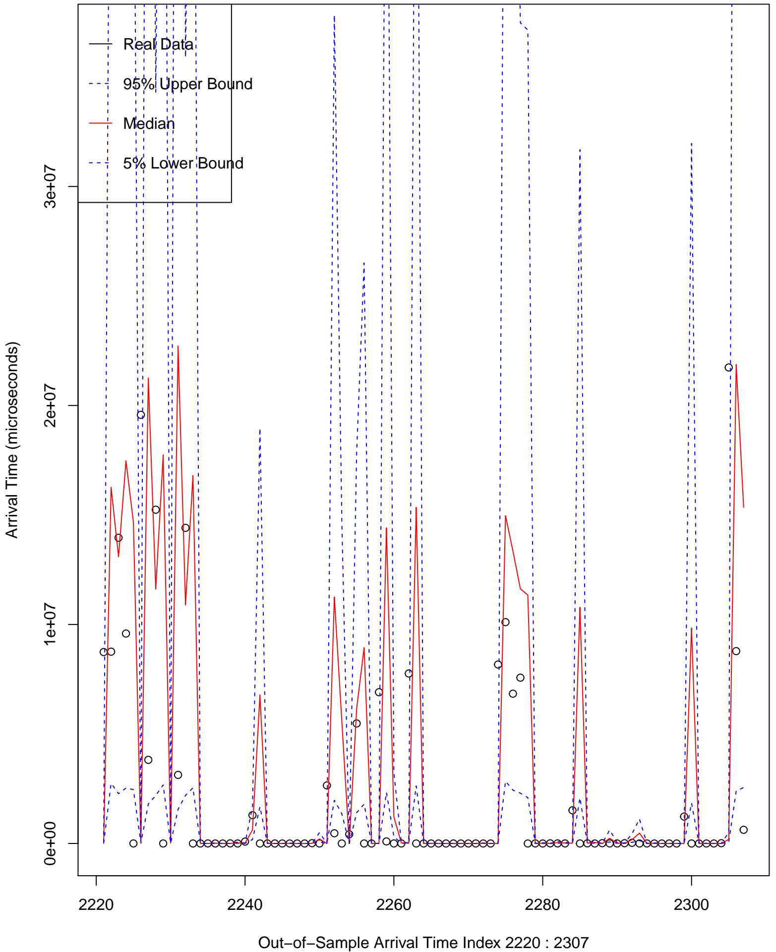
Real Vs Predicted Arrival Time, # States= 5 , Last 30 mins, Stock A
