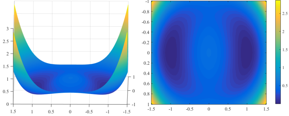
Figure 5: Function landscape of (1.1) for \mathbf{x} = [1; 0] and m \rightarrow \infty for the masked Fourier transform measurements (coded diffraction model [CLS15a]). The landscape is qualitatively similar to that for the Gaussian model (Figure 2).
