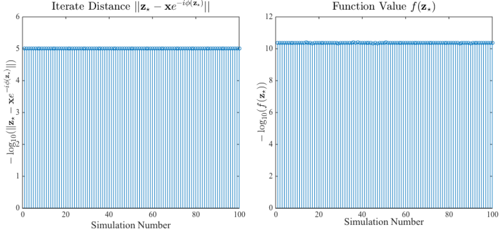
Figure 1: Gradient descent with random initialization seems to always return a global solution for (1.1)! Here n = 100 , m = 5n \log n , step size \mu = 0.05 , and stopping criterion is \|\nabla_z f(z)\| \leq 10^{-5} . We fix the set of random measurements and the ground-truth signal x . The experiments are repeated for 100 times with independent random initializations. z_* denotes the final iterate at convergence. (Left) Final distance to the target; (Right) Final function value (0 if globally optimized). Both vertical axes are on -\log_{10}(\cdot) scale.
