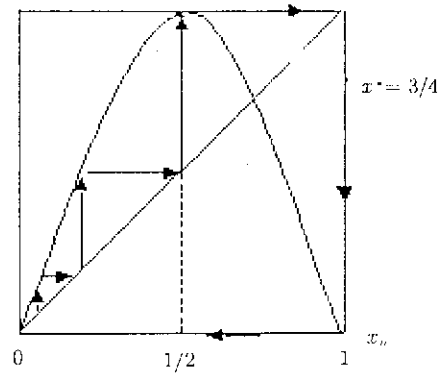
Fig. 1 The homoclinic orbit in map Eq. (1).
