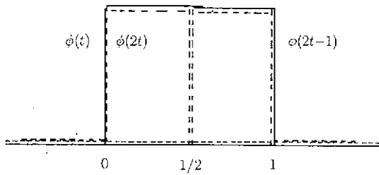
Fig. 2 Haar father wavelet.
