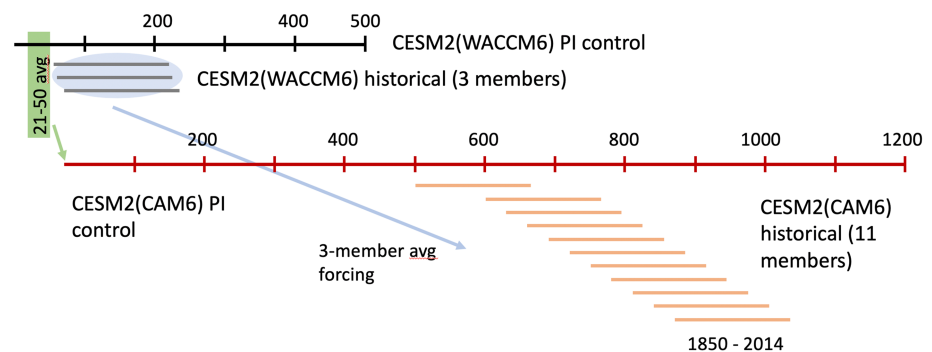
Figure 4. Schematic of the CESM2 PI control and historical simulations. CESM2(WACCM6) PI simulation was started first (black) to obtain the forcing data sets used for the CESM2(CAM6) PI integration (red). These forcings were based on the average of Years 21–50 (green shading). Three historical CESM2(WACCM6) simulations were started from Years 56, 61, and 71 of the corresponding PI simulation (gray lines). As described in section 5, three-member ensemble averages of these WACCM6 simulations (blue shading) were then used to obtain the forcings needed for the CESM2 (CAM6) historical simulations (orange lines). The CESM2(CAM6) historical simulations started from Years 501, 601, 631, 661, 691, 721, 751, 781, 811, 841, and 871 of the corresponding PI simulation. The black and red tick marks indicate 100-year intervals.
