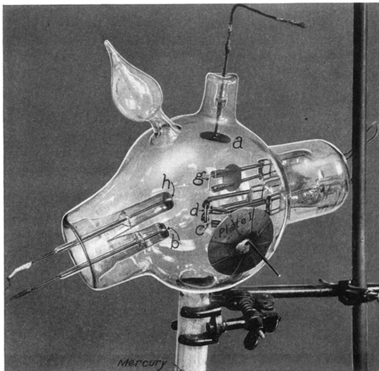
Fig. 1. Experimental tube.
