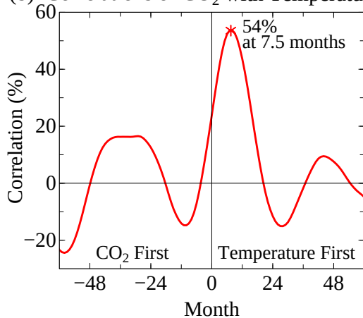
(b) Correlations of CO 2 with Temperature
