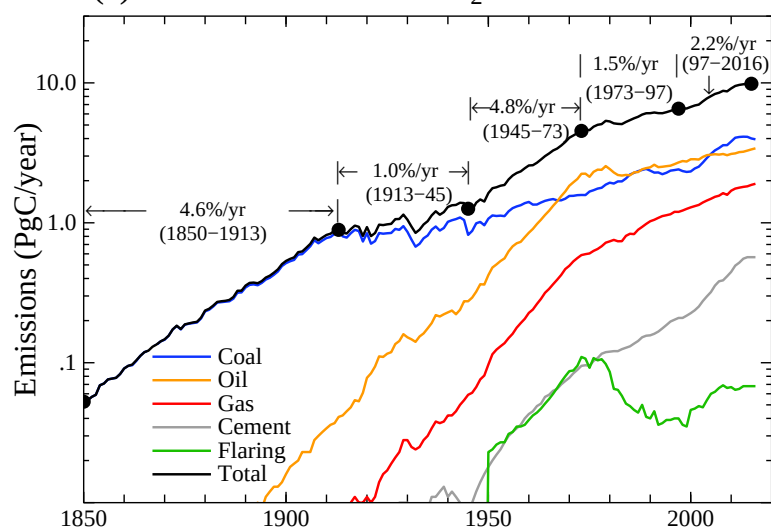
(a) Global Fossil-Fuel CO 2 Annual Emissions
