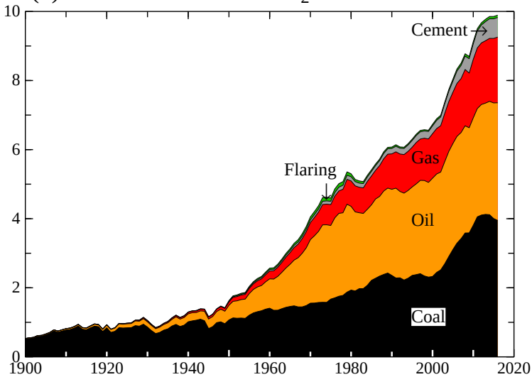
(b) Global Fossil-Fuel CO 2 Annual Emissions
