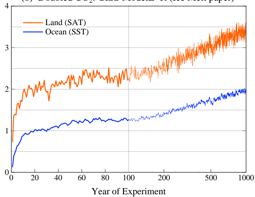
(b) Doubled CO 2 : GISS ModelE-R (Ice Melt paper)
