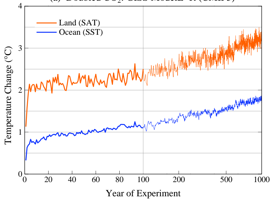
(a) Doubled CO 2 : GISS ModelE-R (CMIP5)
