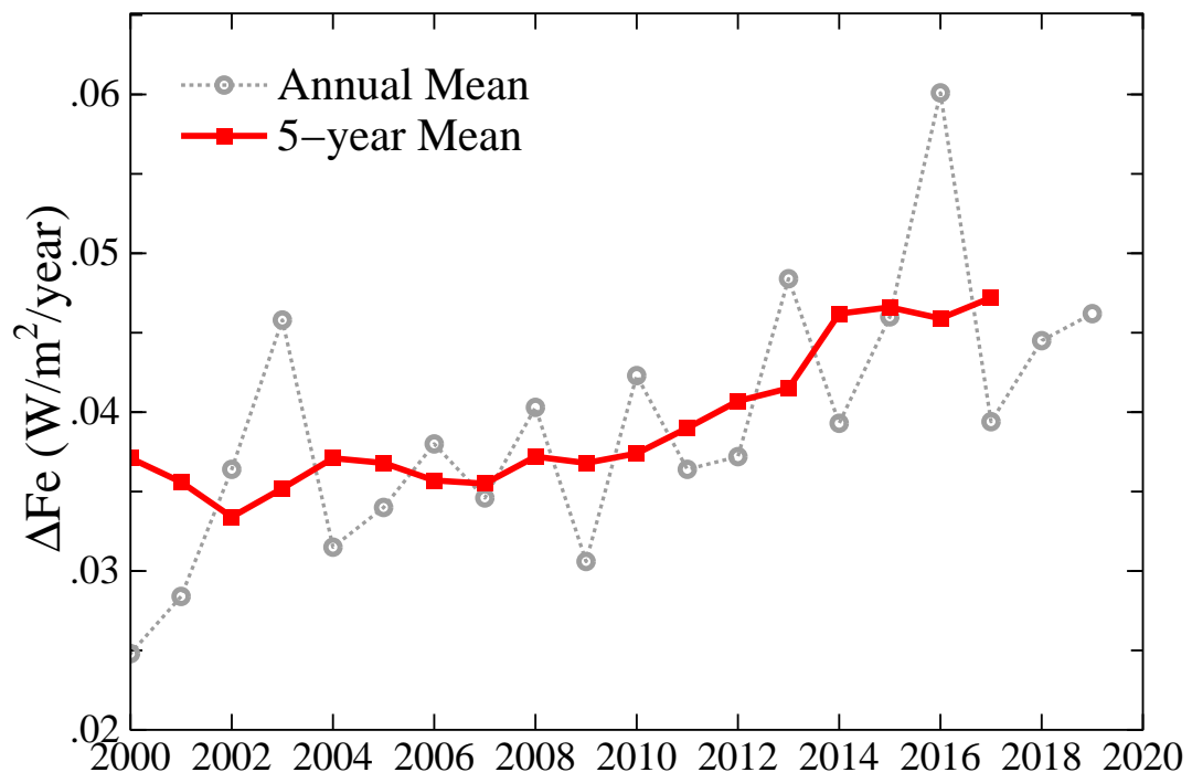
Greenhouse Gas Climate Forcing Growth Rate
