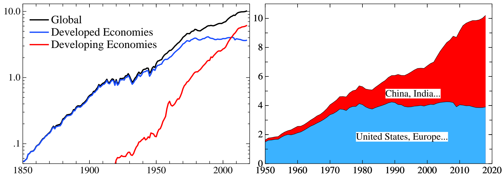
Global Emissions (GtC/Year)
