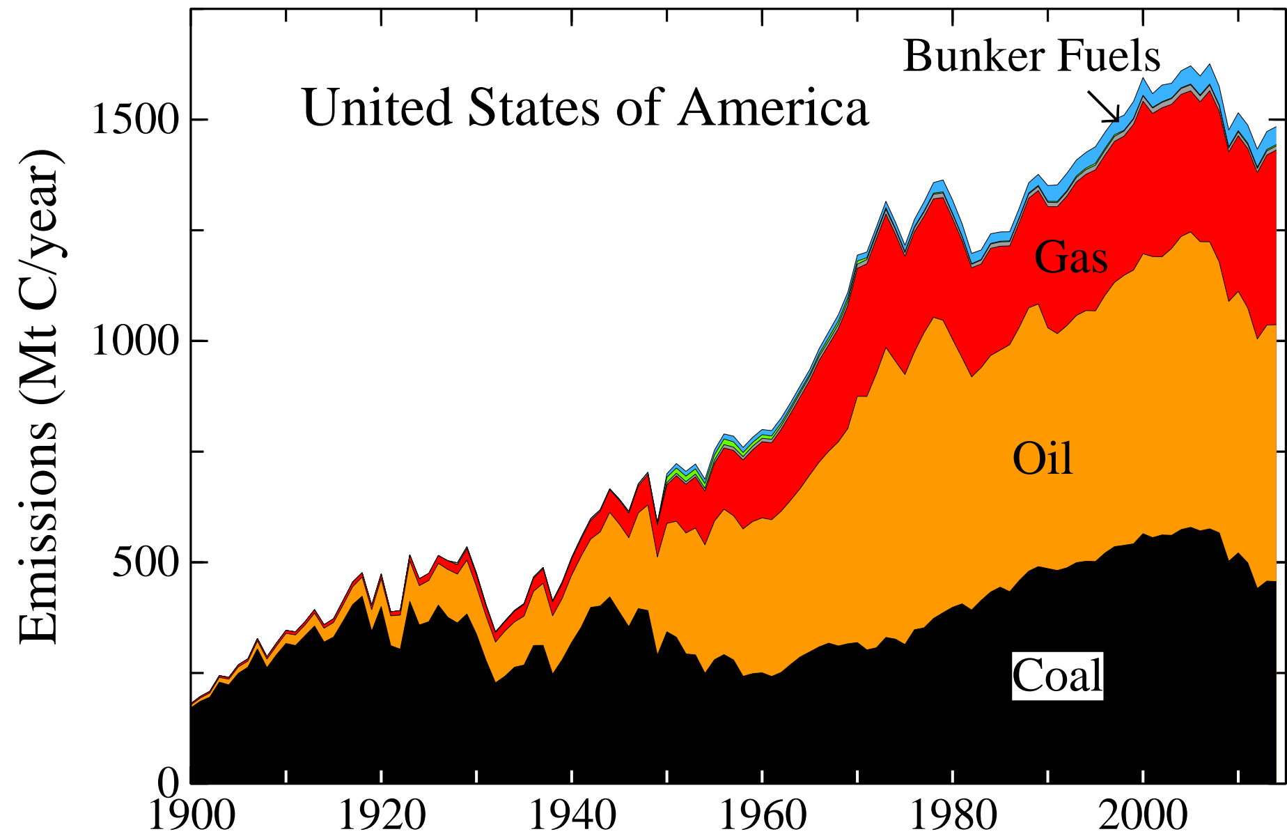
(b) Annual CO 2 Emissions
