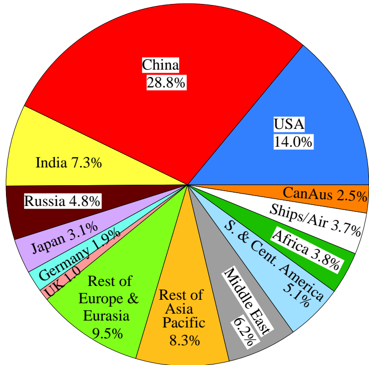
(a) 2018 Annual Emissions (10.2 GtC/yr)
