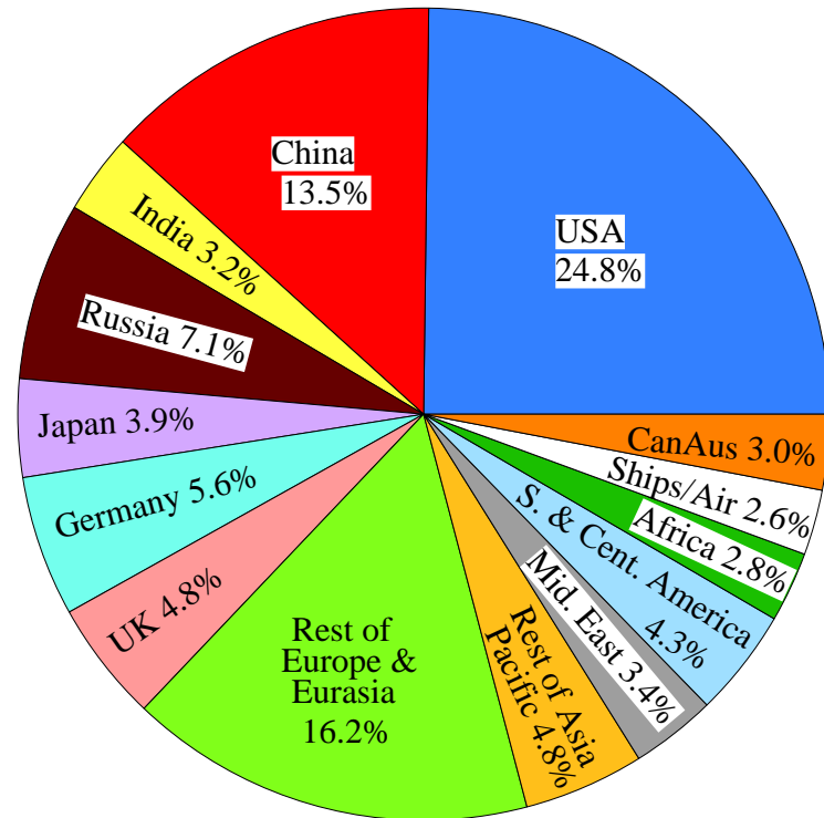
(b) 1751–2018 Cumulative Emissions (442 GtC)
