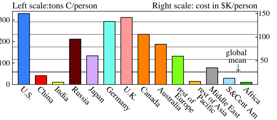
(b) 1751–2018 Cumulative Emissions
