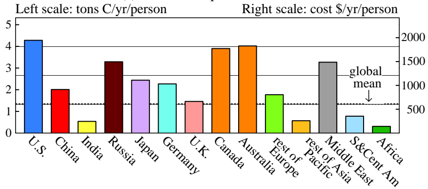
(a) 2018 Per Capita Emissions
