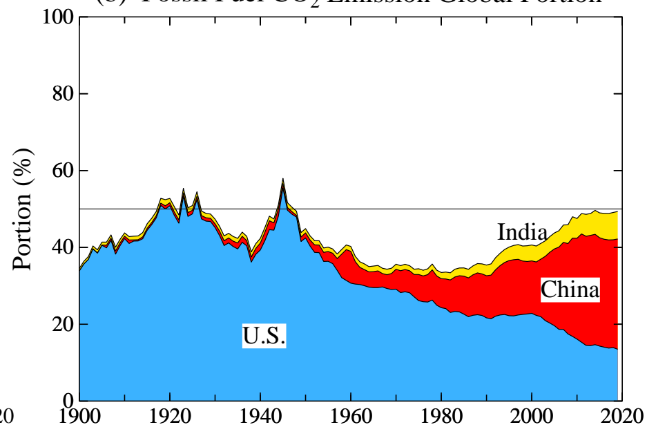
(b) Fossil Fuel CO 2 Emission Global Portion
