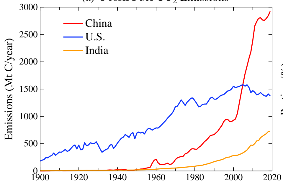
(a) Fossil Fuel CO 2 Emissions
