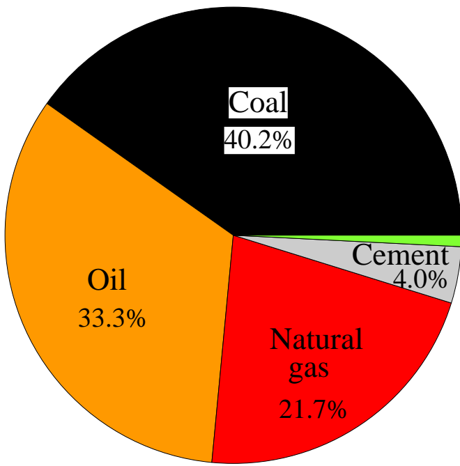
2020 Annual Emissions
