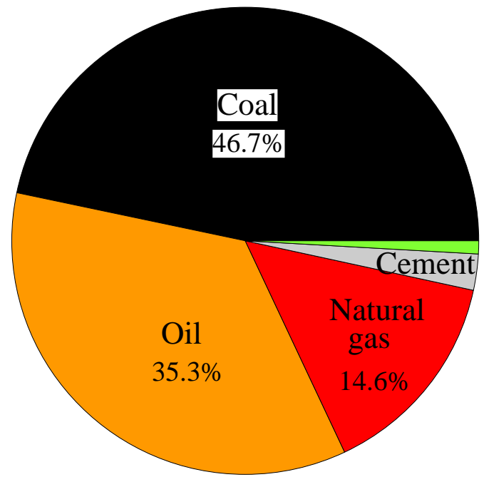
1751–2020 Cumulative Emissions
